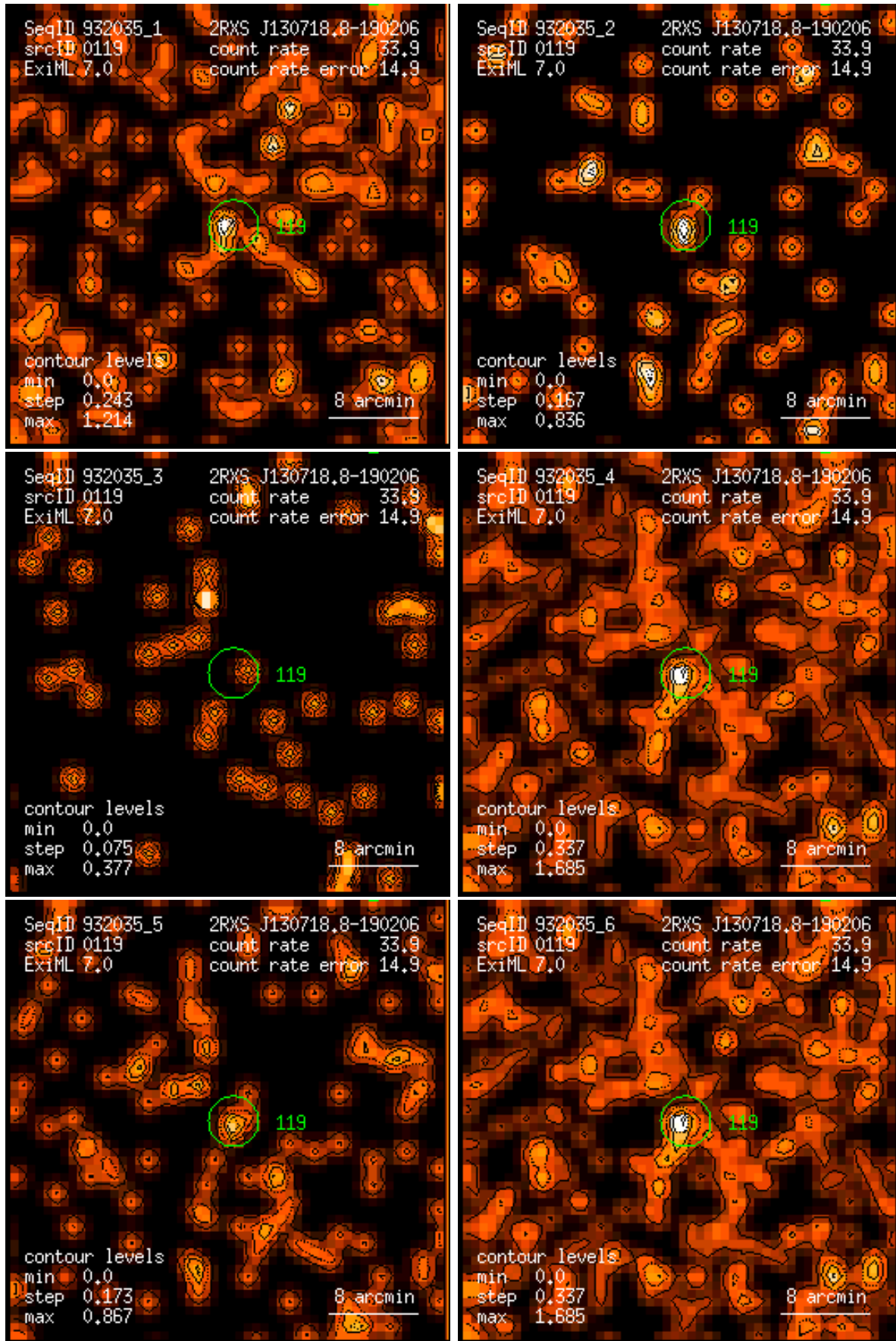
Figure 119: RASS 932035: detection 0119: band rate images, Gaussian filter: (1) PSPC channels 11 – 41, (2) 52 – 90, (3) 91 – 201, (4) 11 – 235, (5) 52 – 201, (6) 11 – 201. Broad band rates in counts/ks. Band rate contour levels in counts/ks/arcmin 2 .
