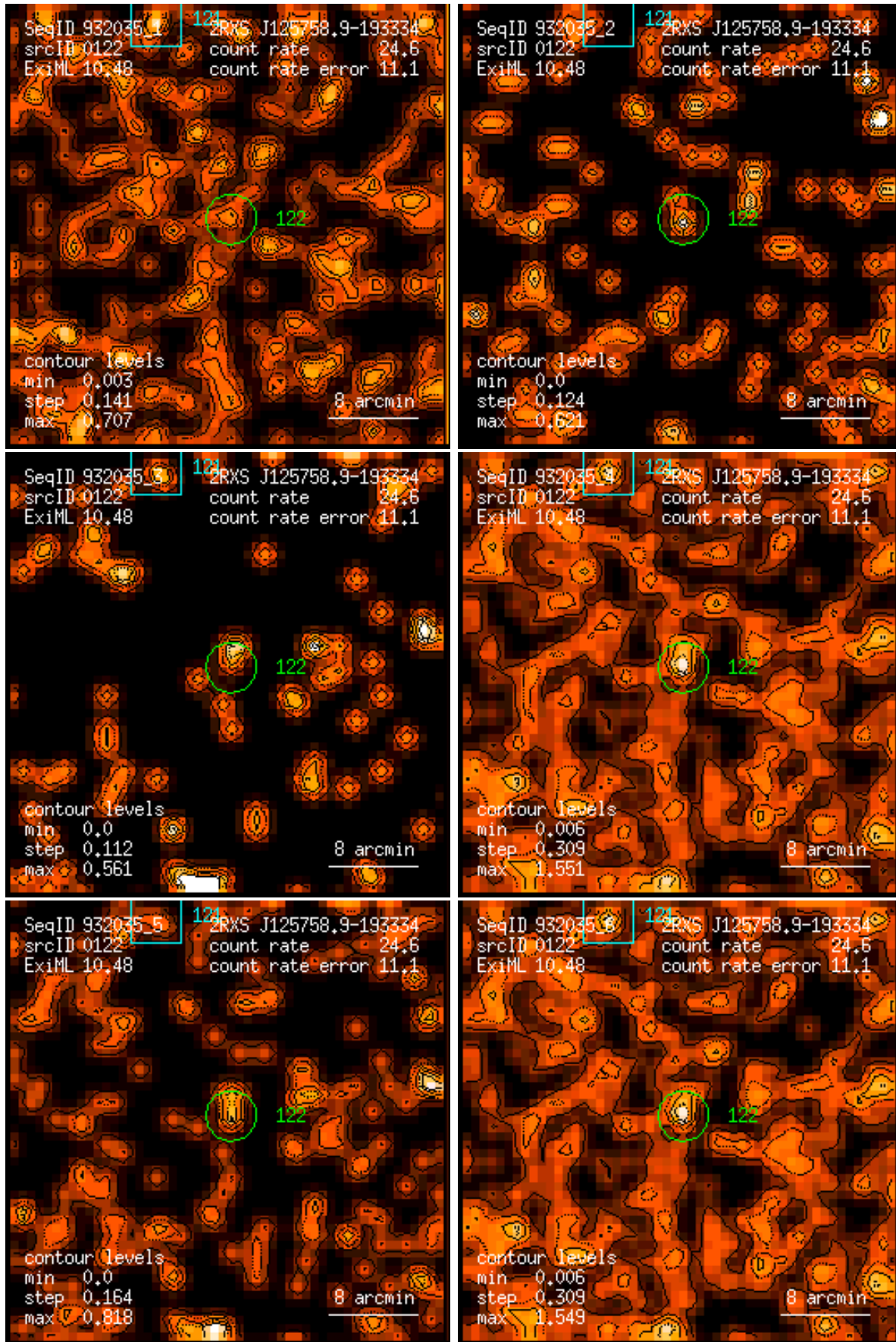
Figure 122: RASS 932035: detection 0122: band rate images, Gaussian filter: (1) PSPC channels 11 – 41, (2) 52 – 90, (3) 91 – 201, (4) 11 – 235, (5) 52 – 201, (6) 11 – 201. Broad band rates in counts/ks. Band rate contour levels in counts/ks/arcmin 2 .
