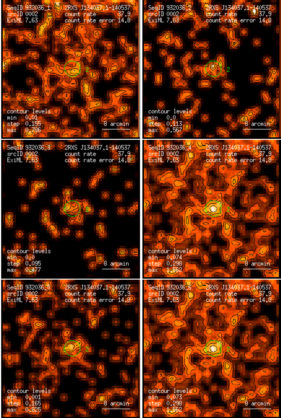
Figure 2: RASS 932036: detection 0002: band rate images, Gaussian filter: (1) PSPC channels 11 – 41, (2) 52 – 90, (3) 91 – 201, (4) 11 – 235, (5) 52 – 201, (6) 11 – 201. Broad band rates in counts/ks. Band rate contour levels in counts/ks/arcmin 2 .
