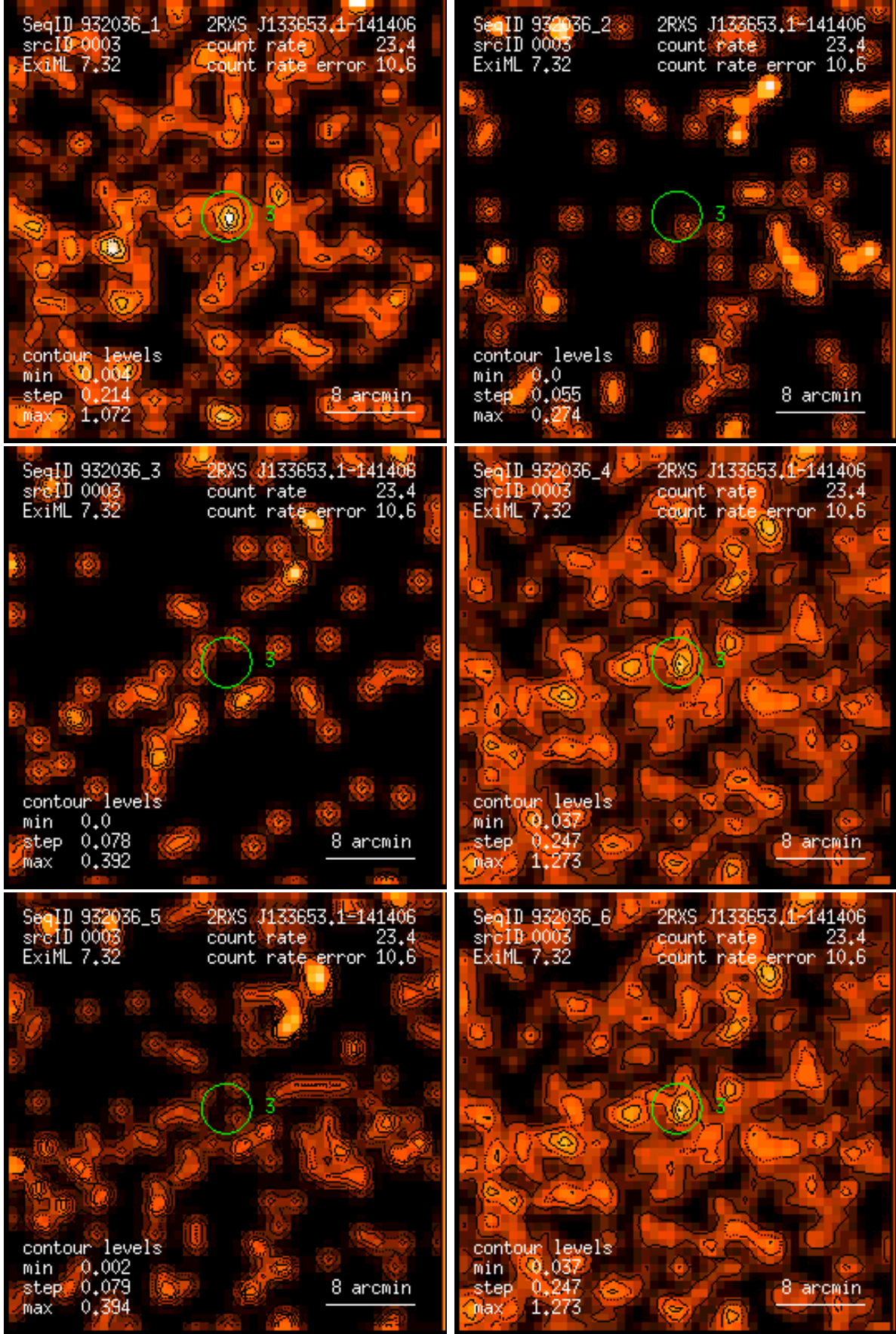
Figure 3: RASS 932036: detection 0003: band rate images, Gaussian filter: (1) PSPC channels 11 – 41, (2) 52 – 90, (3) 91 – 201, (4) 11 – 235, (5) 52 – 201, (6) 11 – 201. Broad band rates in counts/ks. Band rate contour levels in counts/ks/arcmin 2 .
