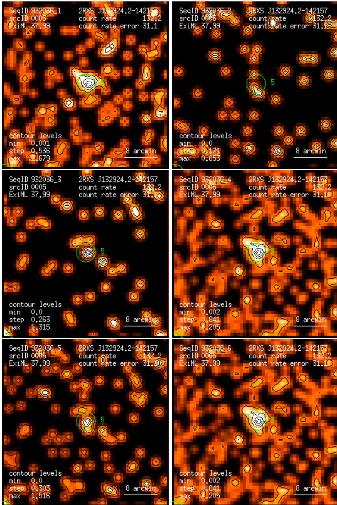
Figure 5: RASS 932036: detection 0005: band rate images, Gaussian filter: (1) PSPC channels 11 – 41, (2) 52 – 90, (3) 91 – 201, (4) 11 – 235, (5) 52 – 201, (6) 11 – 201. Broad band rates in counts/ks. Band rate contour levels in counts/ks/arcmin 2 .
