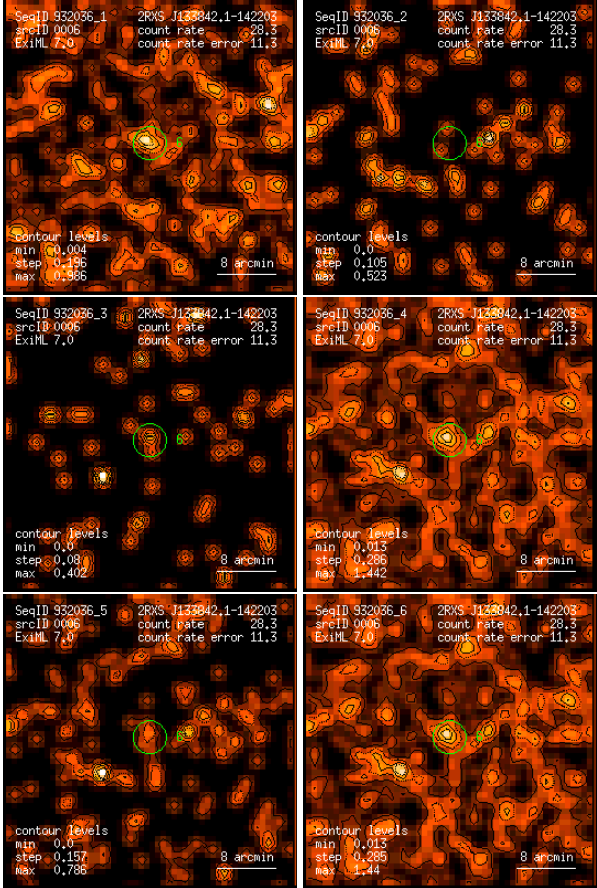
Figure 6: RASS 932036: detection 0006: band rate images, Gaussian filter: (1) PSPC channels 11 – 41, (2) 52 – 90, (3) 91 – 201, (4) 11 – 235, (5) 52 – 201, (6) 11 – 201. Broad band rates in counts/ks. Band rate contour levels in counts/ks/arcmin 2 .
