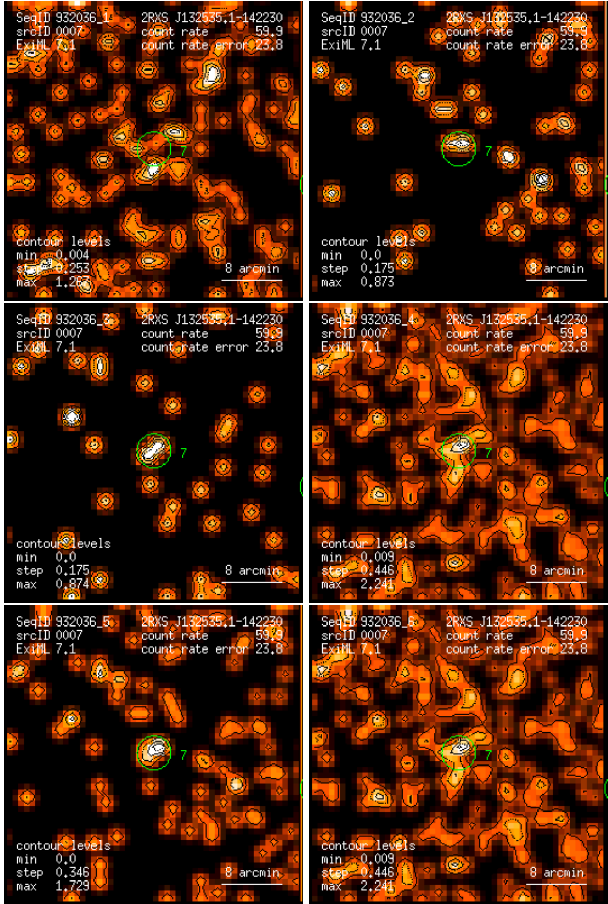
Figure 7: RASS 932036: detection 0007: band rate images, Gaussian filter: (1) PSPC channels 11 – 41, (2) 52 – 90, (3) 91 – 201, (4) 11 – 235, (5) 52 – 201, (6) 11 – 201. Broad band rates in counts/ks. Band rate contour levels in counts/ks/arcmin 2 .
