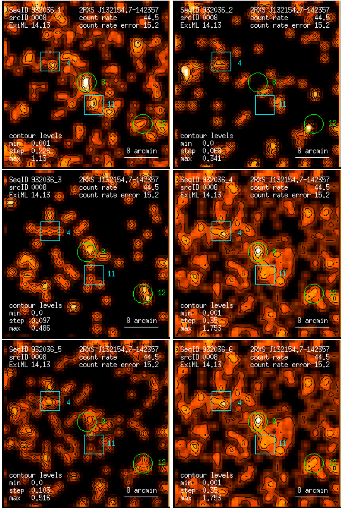
Figure 8: RASS 932036: detection 0008: band rate images, Gaussian filter: (1) PSPC channels 11 – 41, (2) 52 – 90, (3) 91 – 201, (4) 11 – 235, (5) 52 – 201, (6) 11 – 201. Broad band rates in counts/ks. Band rate contour levels in counts/ks/arcmin 2 .
