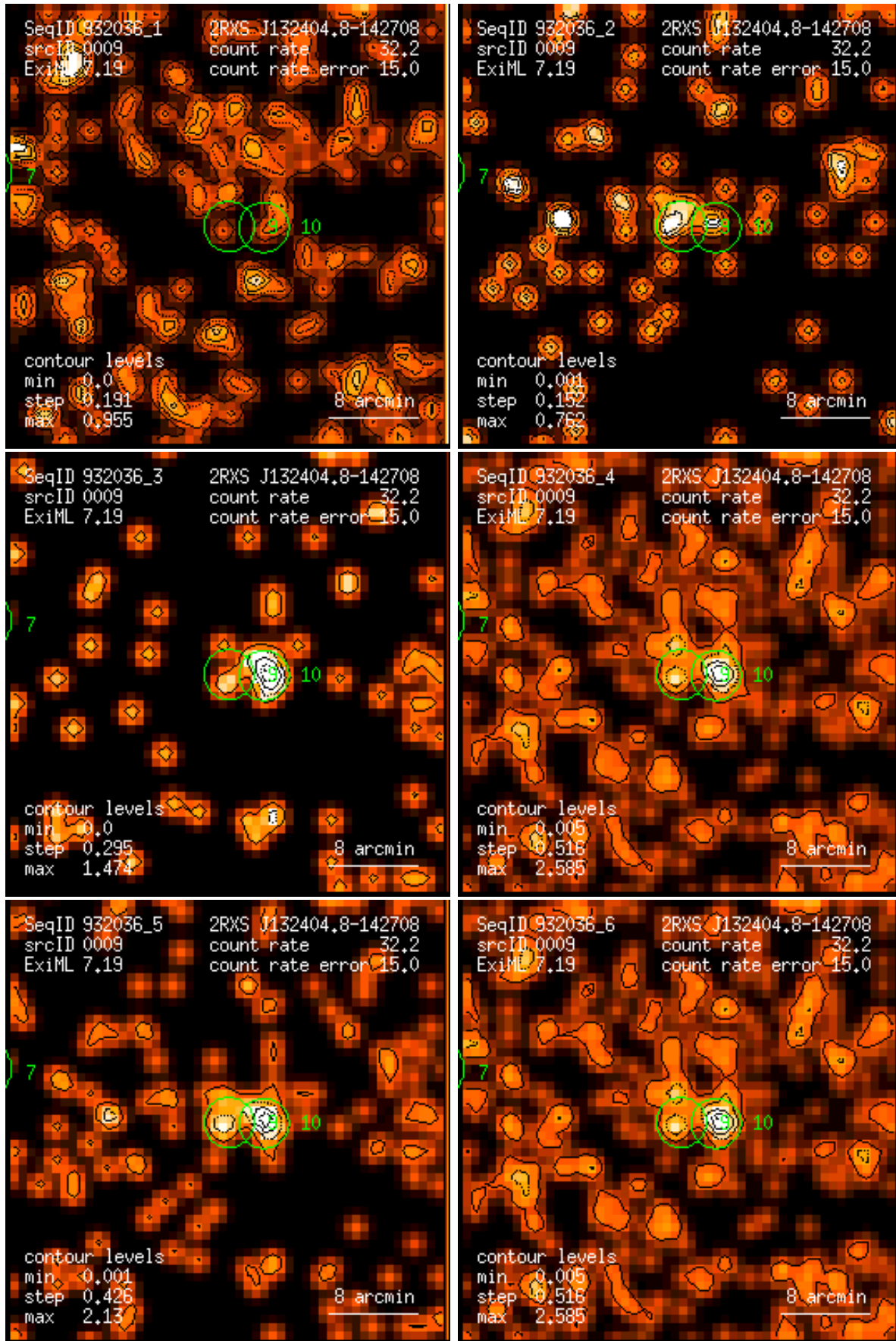
Figure 9: RASS 932036: detection 0009: band rate images, Gaussian filter: (1) PSPC channels 11 – 41, (2) 52 – 90, (3) 91 – 201, (4) 11 – 235, (5) 52 – 201, (6) 11 – 201. Broad band rates in counts/ks. Band rate contour levels in counts/ks/arcmin 2 .
