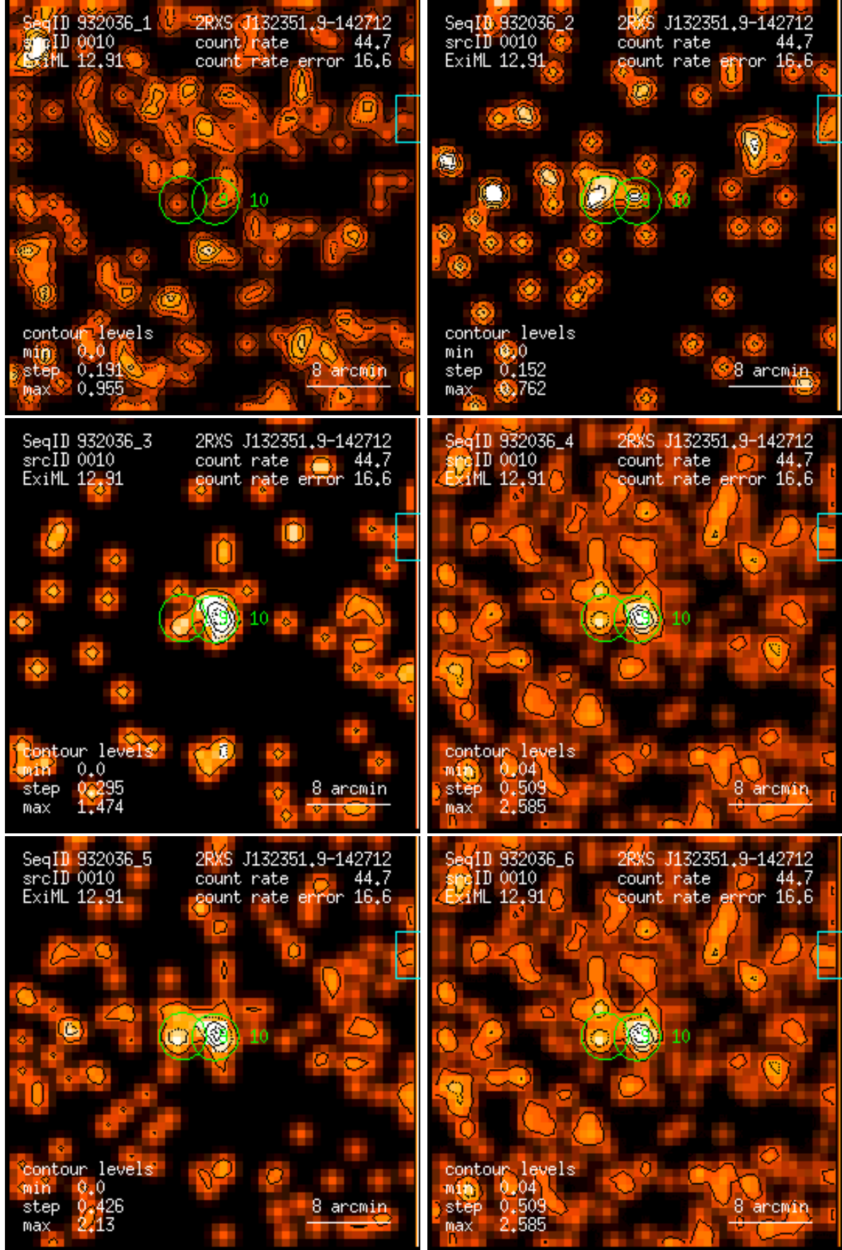
Figure 10: RASS 932036: detection 0010: band rate images, Gaussian filter: (1) PSPC channels 11 – 41, (2) 52 – 90, (3) 91 – 201, (4) 11 – 235, (5) 52 – 201, (6) 11 – 201. Broad band rates in counts/ks. Band rate contour levels in counts/ks/arcmin 2 .
