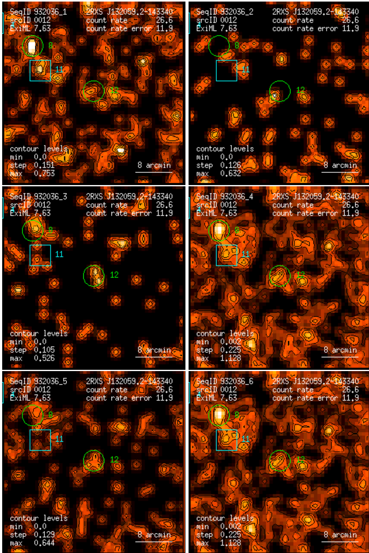
Figure 12: RASS 932036: detection 0012: band rate images, Gaussian filter: (1) PSPC channels 11 – 41, (2) 52 – 90, (3) 91 – 201, (4) 11 – 235, (5) 52 – 201, (6) 11 – 201. Broad band rates in counts/ks. Band rate contour levels in counts/ks/arcmin 2 .
