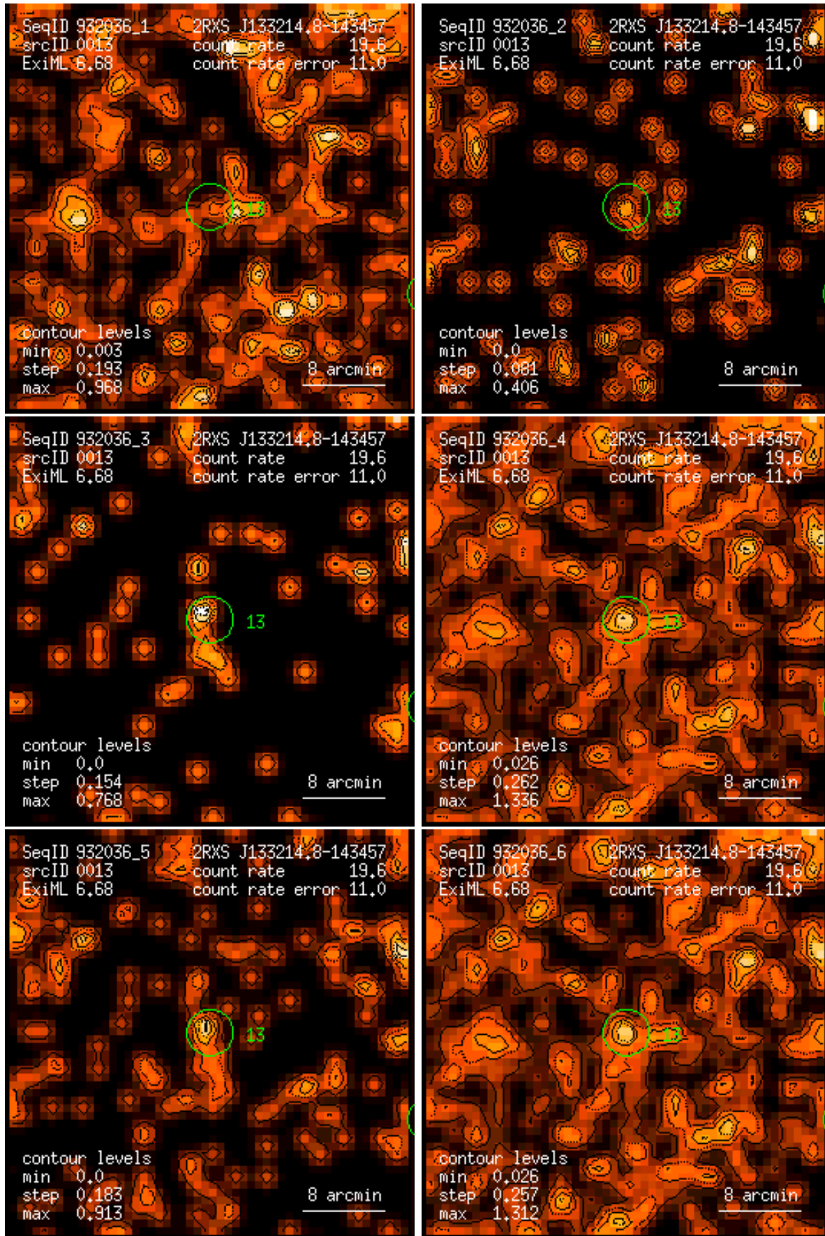
Figure 13: RASS 932036: detection 0013: band rate images, Gaussian filter: (1) PSPC channels 11 – 41, (2) 52 – 90, (3) 91 – 201, (4) 11 – 235, (5) 52 – 201, (6) 11 – 201. Broad band rates in counts/ks. Band rate contour levels in counts/ks/arcmin 2 .
