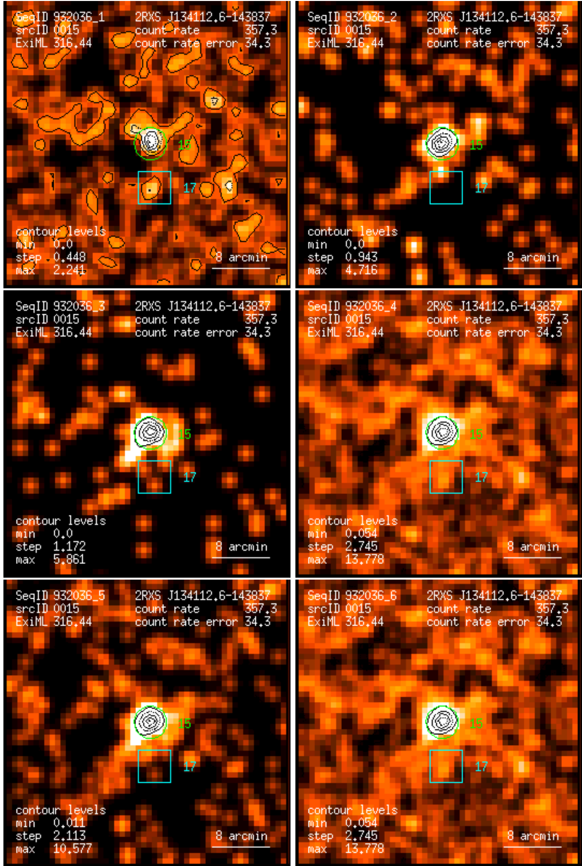
Figure 15: RASS 932036: detection 0015: band rate images, Gaussian filter: (1) PSPC channels 11 – 41, (2) 52 – 90, (3) 91 – 201, (4) 11 – 235, (5) 52 – 201, (6) 11 – 201. Broad band rates in counts/ks. Band rate contour levels in counts/ks/arcmin 2 .
