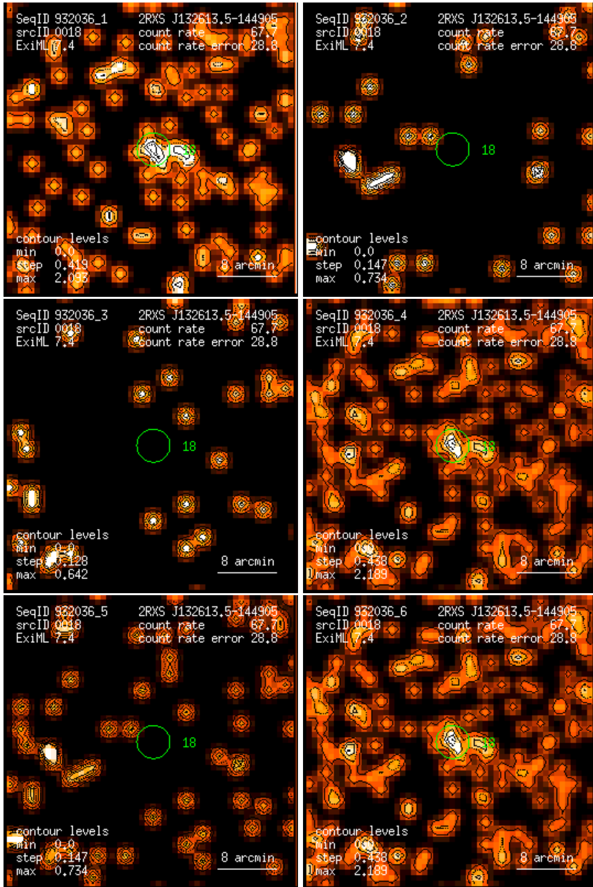
Figure 18: RASS 932036: detection 0018: band rate images, Gaussian filter: (1) PSPC channels 11 – 41, (2) 52 – 90, (3) 91 – 201, (4) 11 – 235, (5) 52 – 201, (6) 11 – 201. Broad band rates in counts/ks. Band rate contour levels in counts/ks/arcmin 2 .
