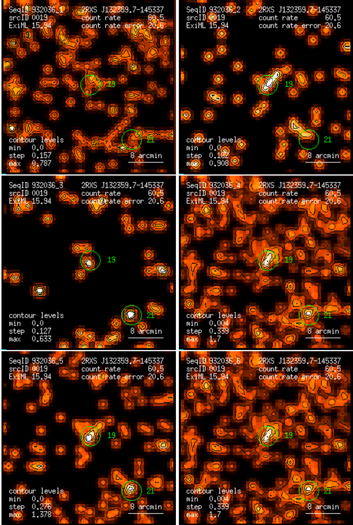
Figure 19: RASS 932036: detection 0019: band rate images, Gaussian filter: (1) PSPC channels 11 – 41, (2) 52 – 90, (3) 91 – 201, (4) 11 – 235, (5) 52 – 201, (6) 11 – 201. Broad band rates in counts/ks. Band rate contour levels in counts/ks/arcmin 2 .
