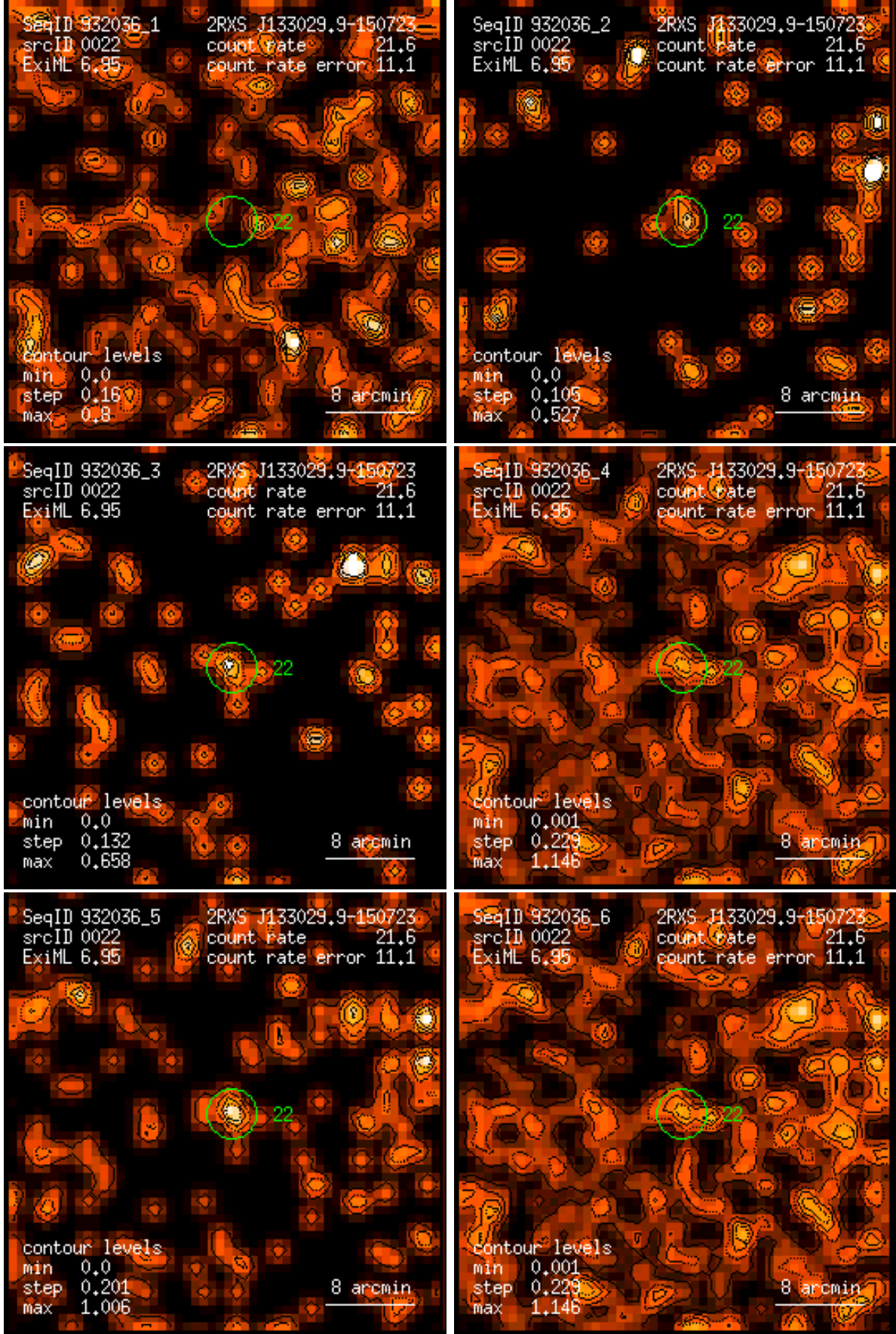
Figure 22: RASS 932036: detection 0022: band rate images, Gaussian filter: (1) PSPC channels 11 – 41, (2) 52 – 90, (3) 91 – 201, (4) 11 – 235, (5) 52 – 201, (6) 11 – 201. Broad band rates in counts/ks. Band rate contour levels in counts/ks/arcmin 2 .
