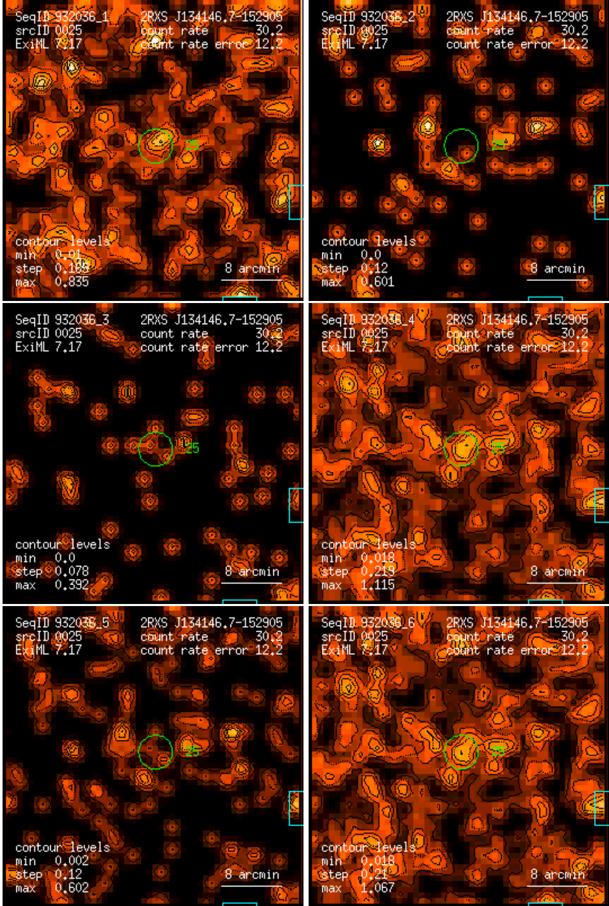
Figure 25: RASS 932036: detection 0025: band rate images, Gaussian filter: (1) PSPC channels 11 – 41, (2) 52 – 90, (3) 91 – 201, (4) 11 – 235, (5) 52 – 201, (6) 11 – 201. Broad band rates in counts/ks. Band rate contour levels in counts/ks/arcmin 2 .
