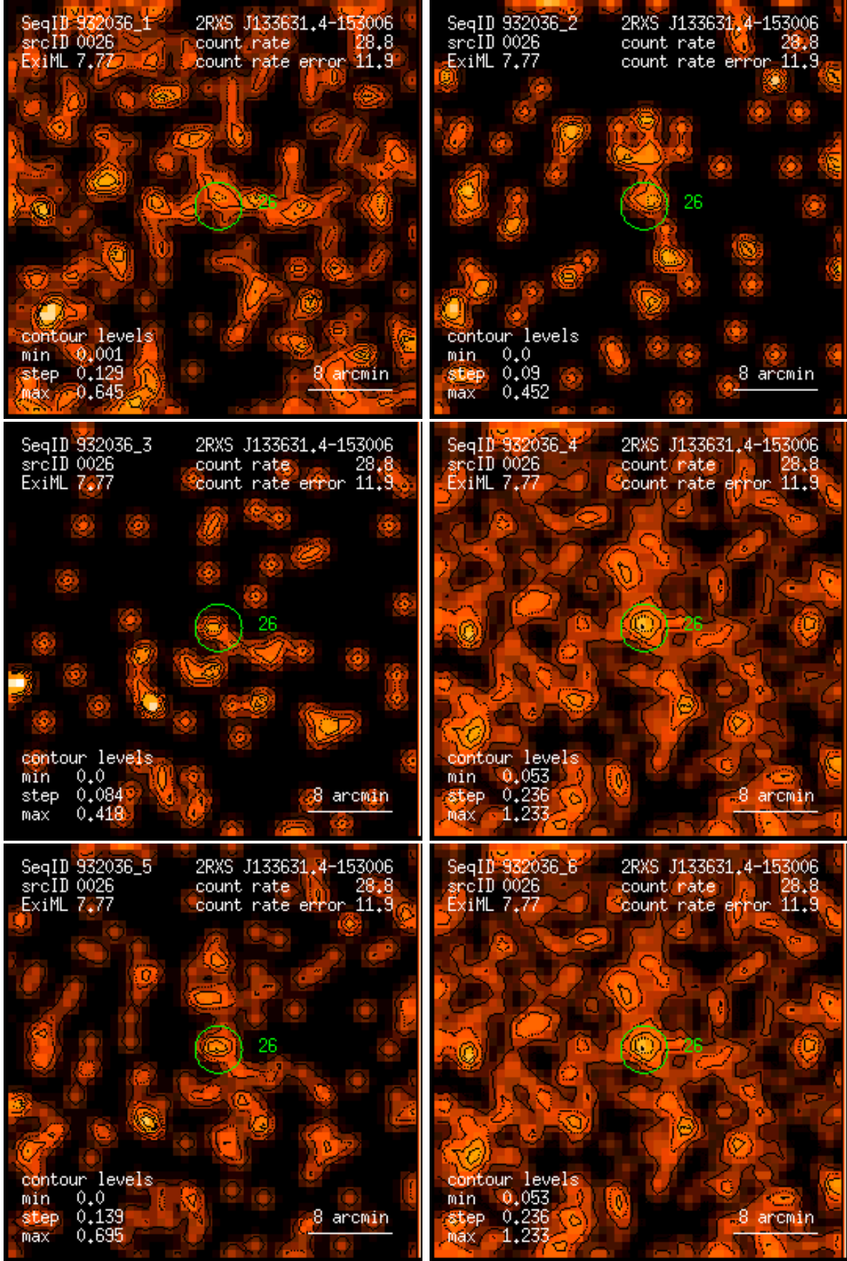
Figure 26: RASS 932036: detection 0026: band rate images, Gaussian filter: (1) PSPC channels 11 – 41, (2) 52 – 90, (3) 91 – 201, (4) 11 – 235, (5) 52 – 201, (6) 11 – 201. Broad band rates in counts/ks. Band rate contour levels in counts/ks/arcmin 2 .
