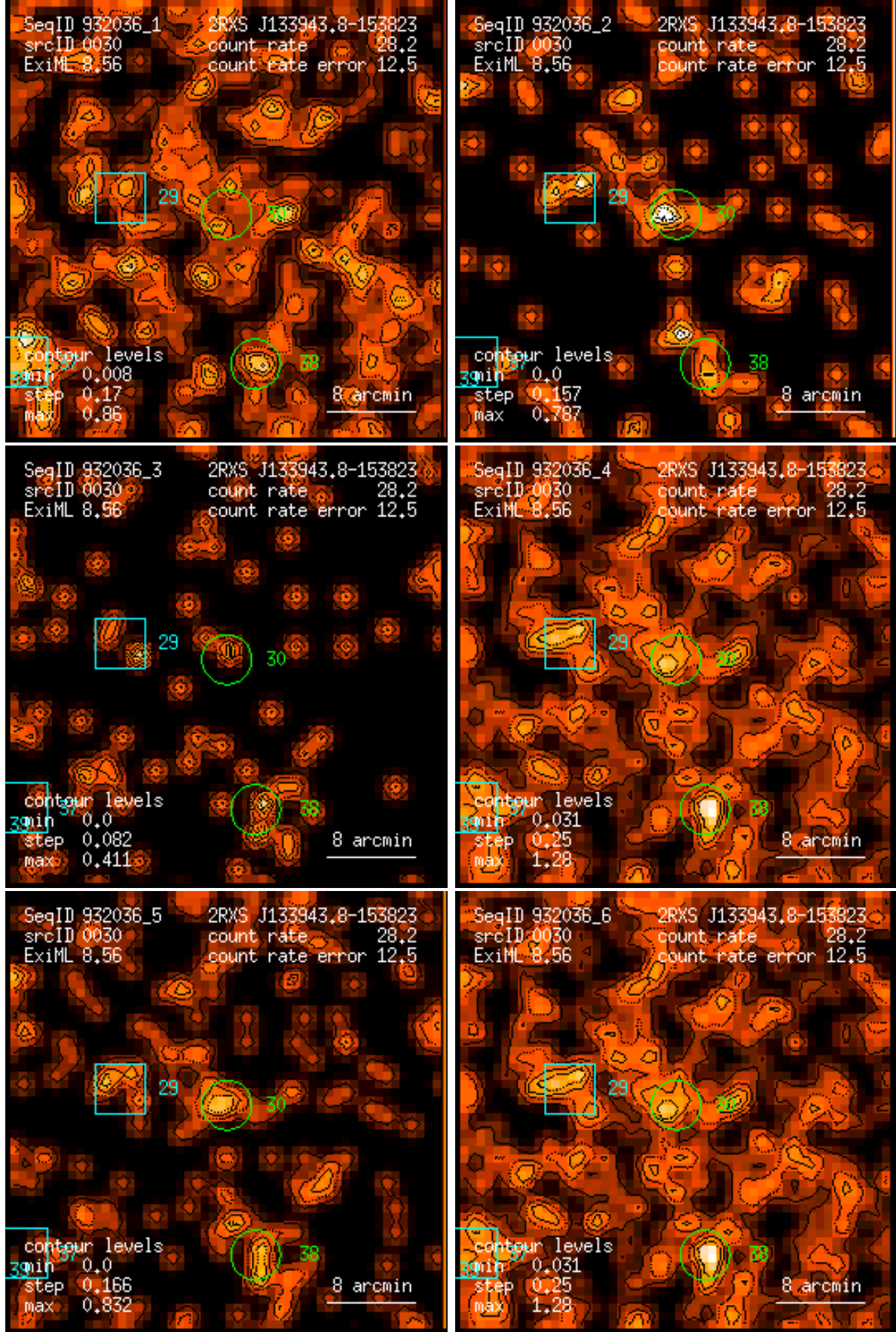
Figure 30: RASS 932036: detection 0030: band rate images, Gaussian filter: (1) PSPC channels 11 – 41, (2) 52 – 90, (3) 91 – 201, (4) 11 – 235, (5) 52 – 201, (6) 11 – 201. Broad band rates in counts/ks. Band rate contour levels in counts/ks/arcmin 2 .
