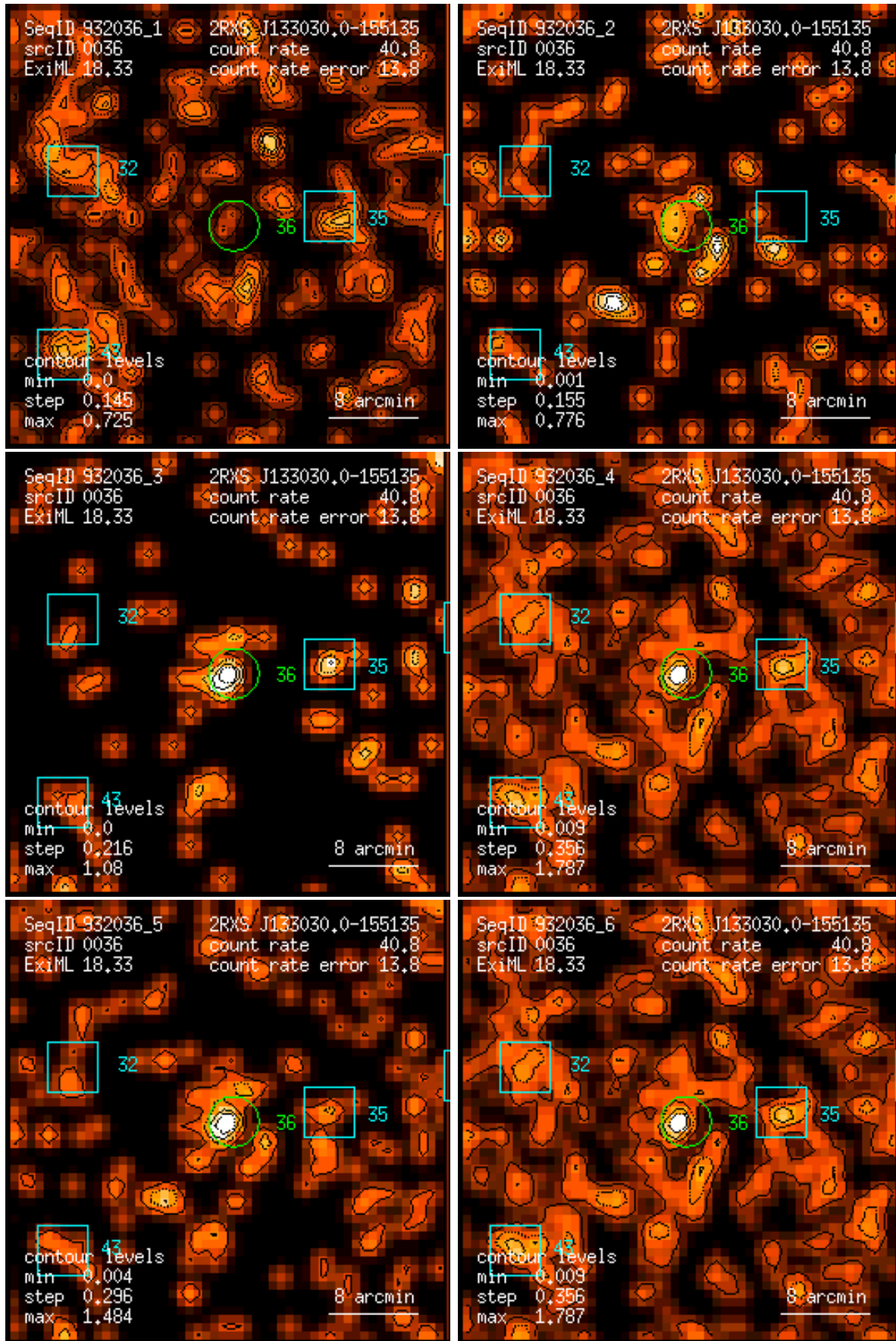
Figure 36: RASS 932036: detection 0036: band rate images, Gaussian filter: (1) PSPC channels 11 – 41, (2) 52 – 90, (3) 91 – 201, (4) 11 – 235, (5) 52 – 201, (6) 11 – 201. Broad band rates in counts/ks. Band rate contour levels in counts/ks/arcmin 2 .
