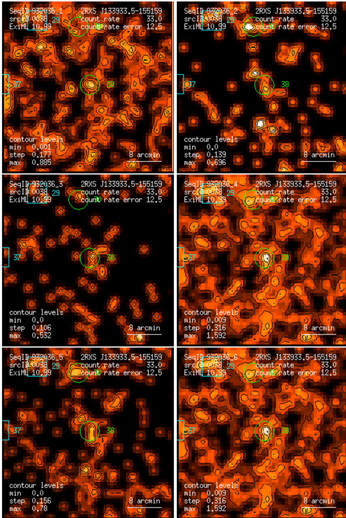
Figure 38: RASS 932036: detection 0038: band rate images, Gaussian filter: (1) PSPC channels 11 – 41, (2) 52 – 90, (3) 91 – 201, (4) 11 – 235, (5) 52 – 201, (6) 11 – 201. Broad band rates in counts/ks. Band rate contour levels in counts/ks/arcmin 2 .
