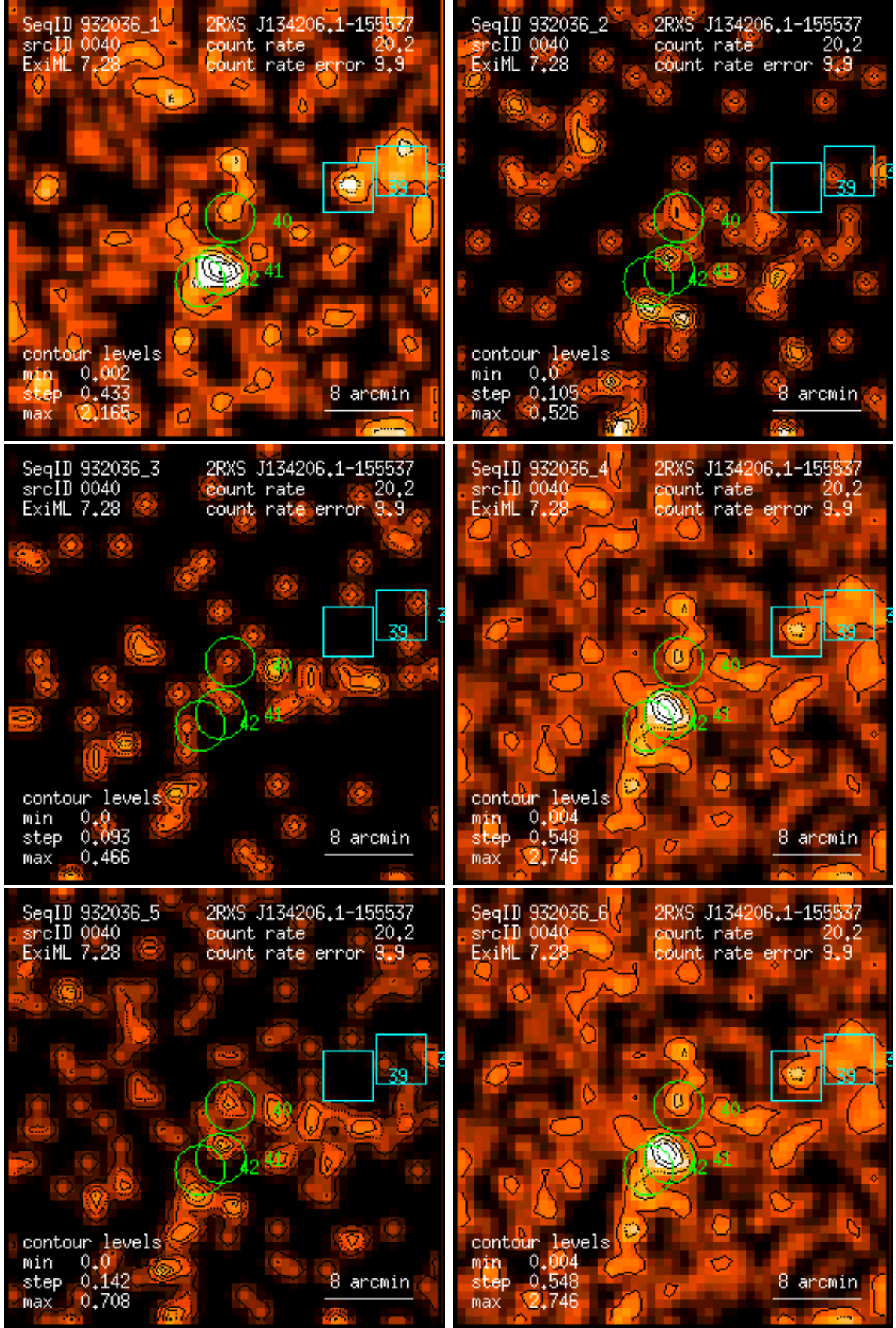
Figure 40: RASS 932036: detection 0040: band rate images, Gaussian filter: (1) PSPC channels 11 – 41, (2) 52 – 90, (3) 91 – 201, (4) 11 – 235, (5) 52 – 201, (6) 11 – 201. Broad band rates in counts/ks. Band rate contour levels in counts/ks/arcmin 2 .
