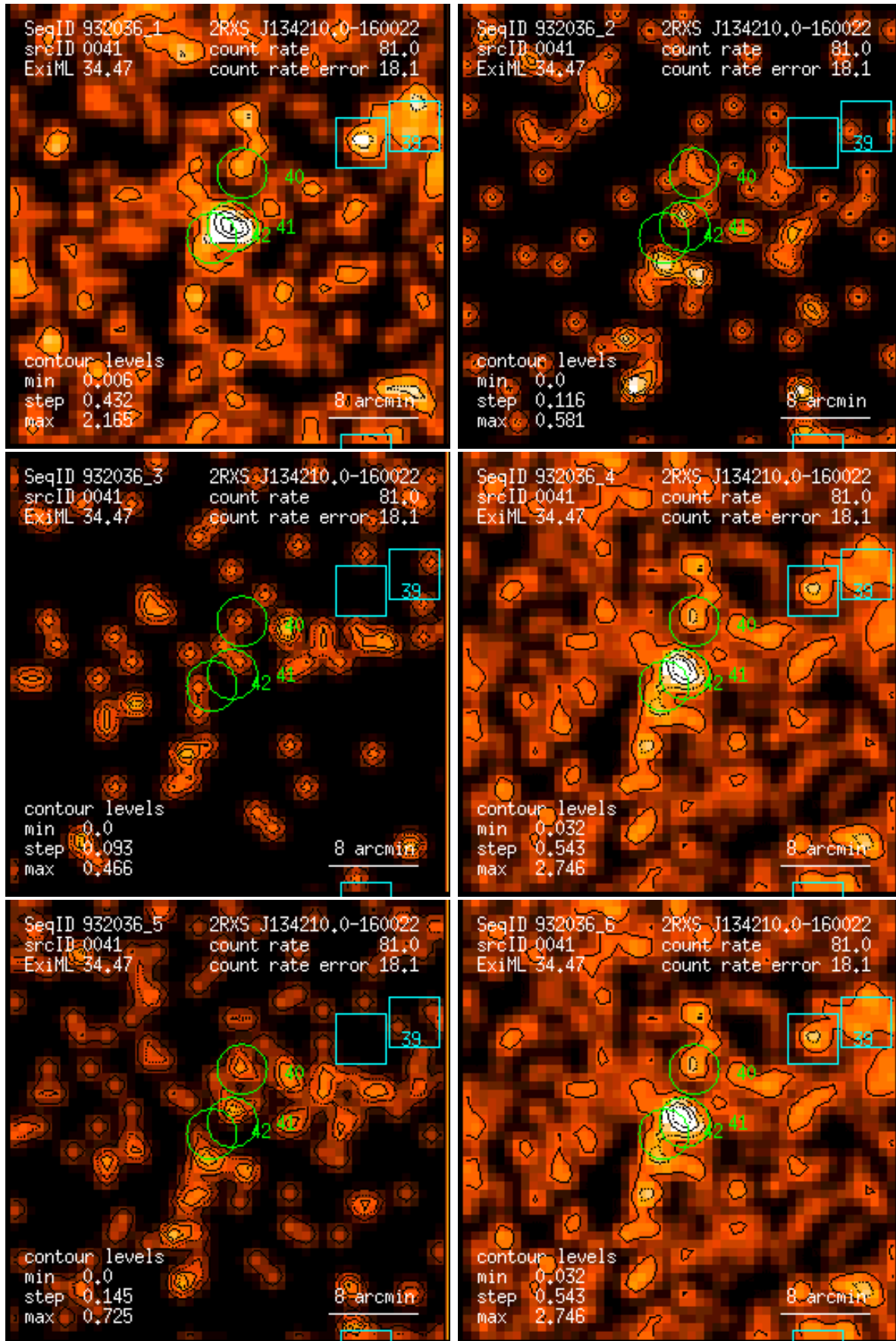
Figure 41: RASS 932036: detection 0041: band rate images, Gaussian filter: (1) PSPC channels 11 – 41, (2) 52 – 90, (3) 91 – 201, (4) 11 – 235, (5) 52 – 201, (6) 11 – 201. Broad band rates in counts/ks. Band rate contour levels in counts/ks/arcmin 2 .
