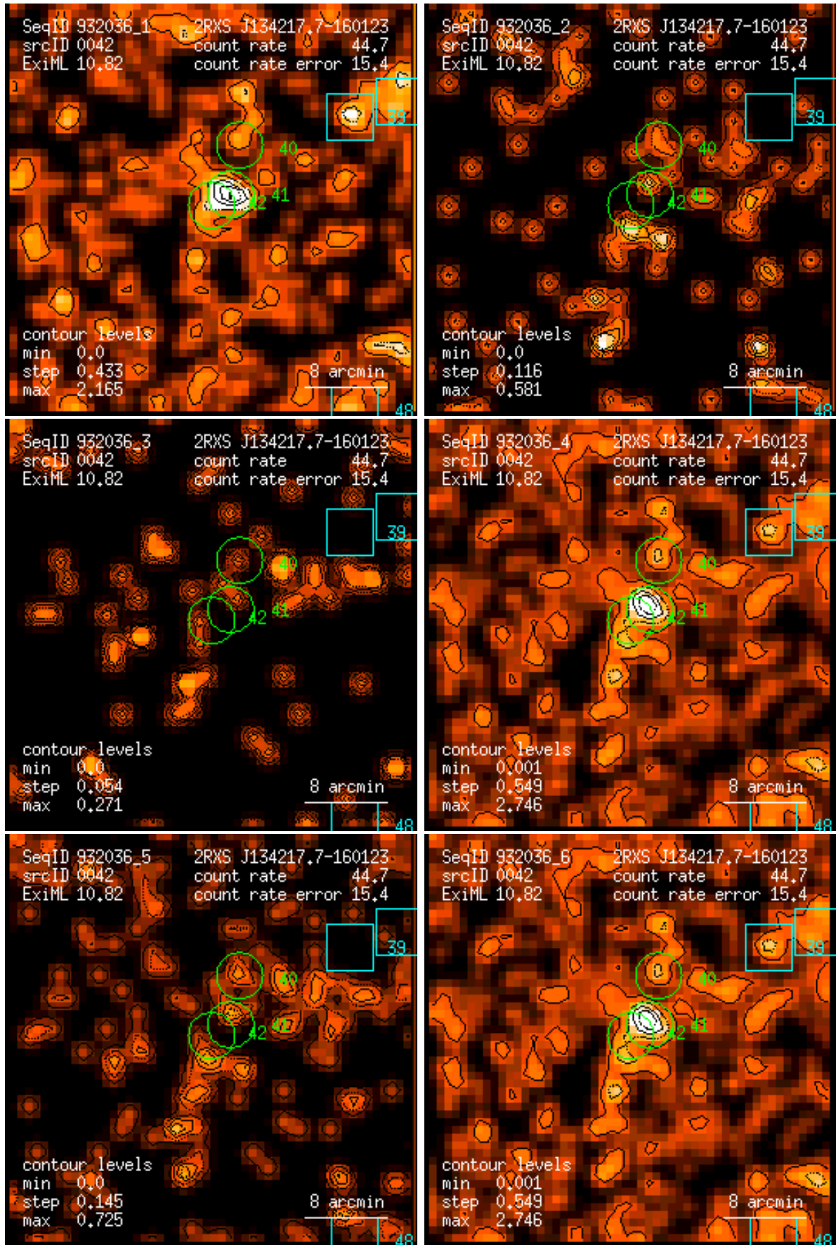
Figure 42: RASS 932036: detection 0042: band rate images, Gaussian filter: (1) PSPC channels 11 – 41, (2) 52 – 90, (3) 91 – 201, (4) 11 – 235, (5) 52 – 201, (6) 11 – 201. Broad band rates in counts/ks. Band rate contour levels in counts/ks/arcmin 2 .
