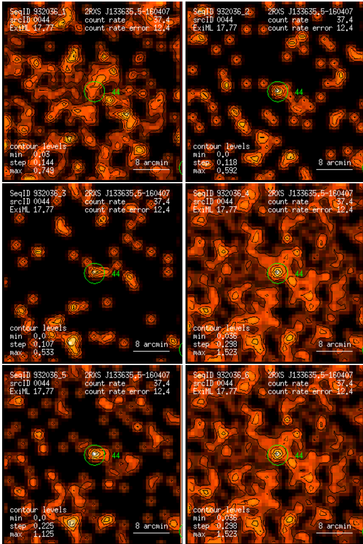
Figure 44: RASS 932036: detection 0044: band rate images, Gaussian filter: (1) PSPC channels 11 – 41, (2) 52 – 90, (3) 91 – 201, (4) 11 – 235, (5) 52 – 201, (6) 11 – 201. Broad band rates in counts/ks. Band rate contour levels in counts/ks/arcmin 2 .
