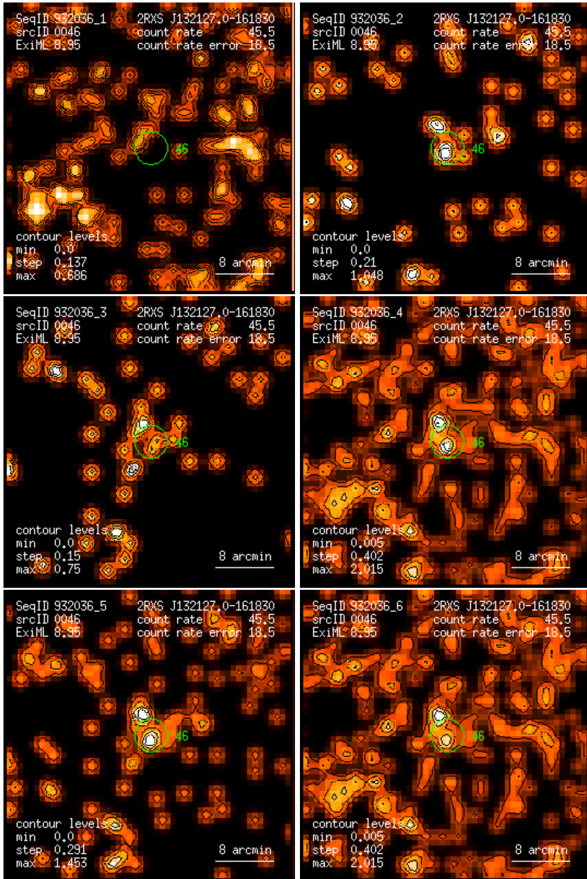
Figure 46: RASS 932036: detection 0046: band rate images, Gaussian filter: (1) PSPC channels 11 – 41, (2) 52 – 90, (3) 91 – 201, (4) 11 – 235, (5) 52 – 201, (6) 11 – 201. Broad band rates in counts/ks. Band rate contour levels in counts/ks/arcmin 2 .
