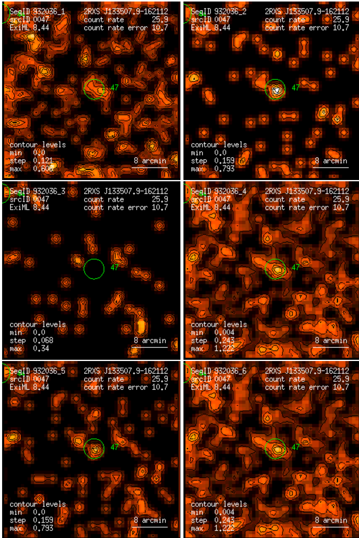
Figure 47: RASS 932036: detection 0047: band rate images, Gaussian filter: (1) PSPC channels 11 – 41, (2) 52 – 90, (3) 91 – 201, (4) 11 – 235, (5) 52 – 201, (6) 11 – 201. Broad band rates in counts/ks. Band rate contour levels in counts/ks/arcmin 2 .
