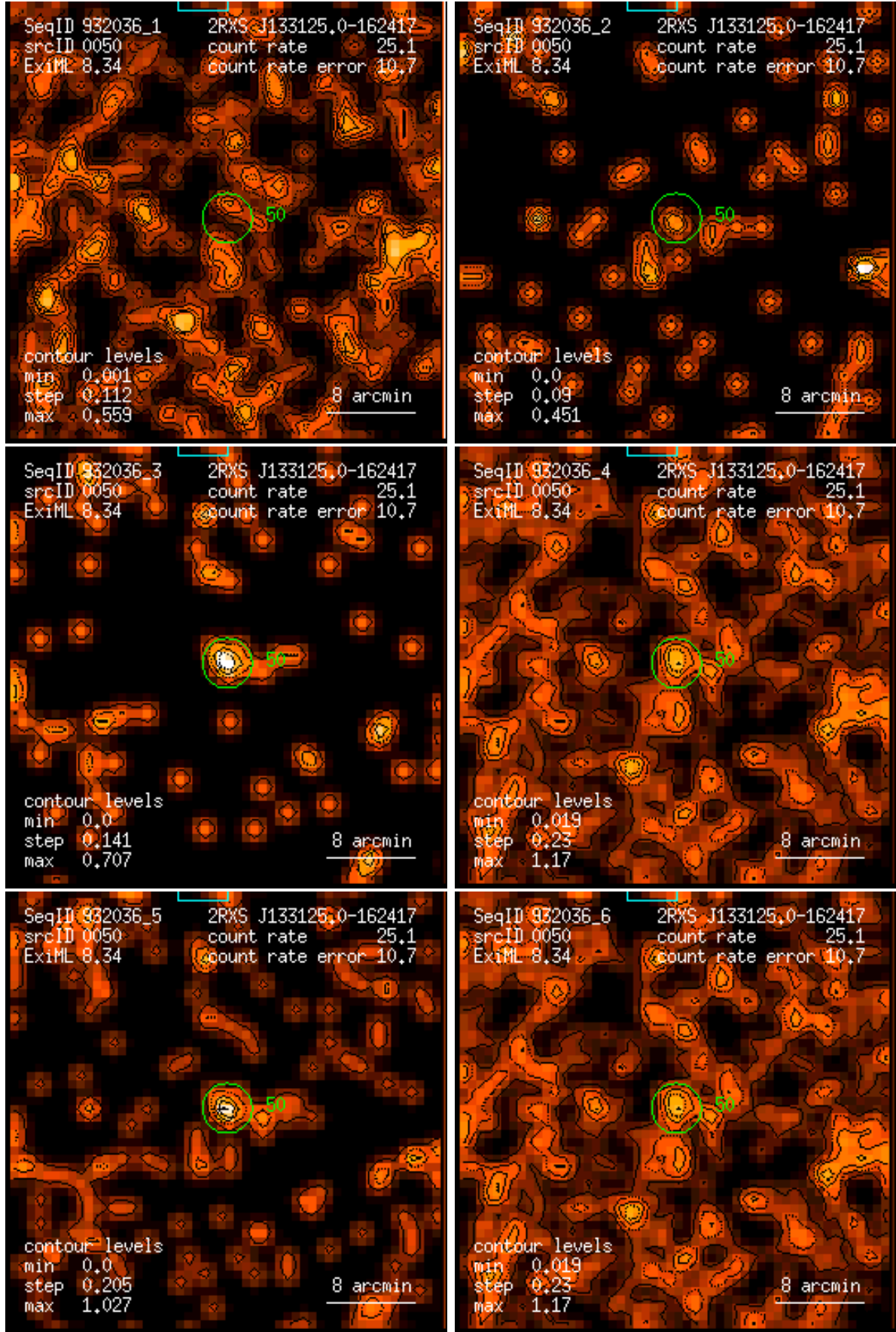
Figure 50: RASS 932036: detection 0050: band rate images, Gaussian filter: (1) PSPC channels 11 – 41, (2) 52 – 90, (3) 91 – 201, (4) 11 – 235, (5) 52 – 201, (6) 11 – 201. Broad band rates in counts/ks. Band rate contour levels in counts/ks/arcmin 2 .
