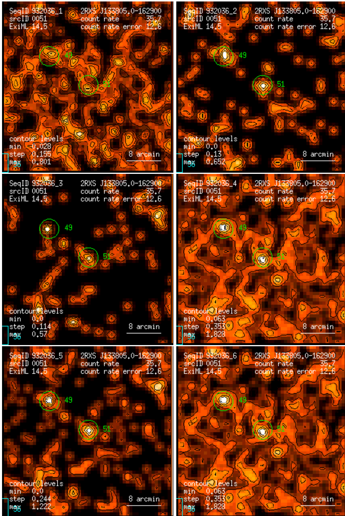
Figure 51: RASS 932036: detection 0051: band rate images, Gaussian filter: (1) PSPC channels 11 – 41, (2) 52 – 90, (3) 91 – 201, (4) 11 – 235, (5) 52 – 201, (6) 11 – 201. Broad band rates in counts/ks. Band rate contour levels in counts/ks/arcmin 2 .
