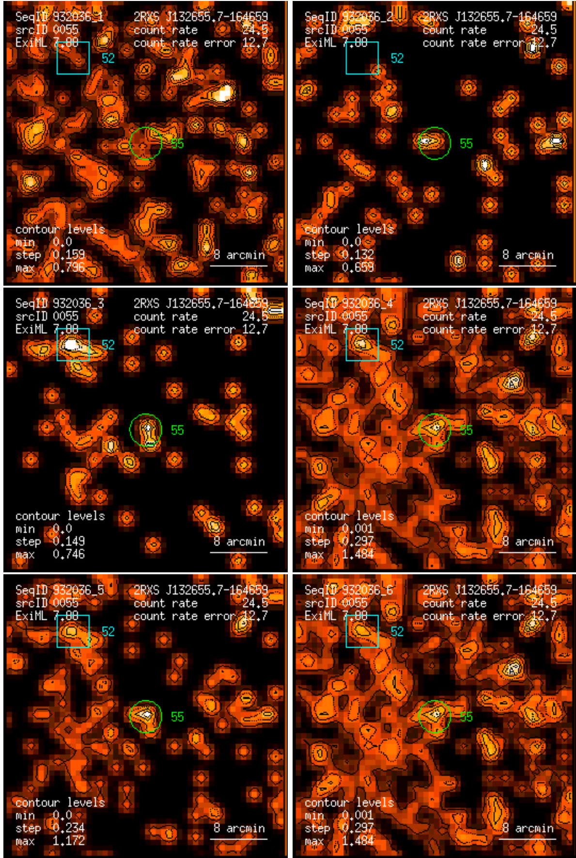
Figure 55: RASS 932036: detection 0055: band rate images, Gaussian filter: (1) PSPC channels 11 – 41, (2) 52 – 90, (3) 91 – 201, (4) 11 – 235, (5) 52 – 201, (6) 11 – 201. Broad band rates in counts/ks. Band rate contour levels in counts/ks/arcmin 2 .
