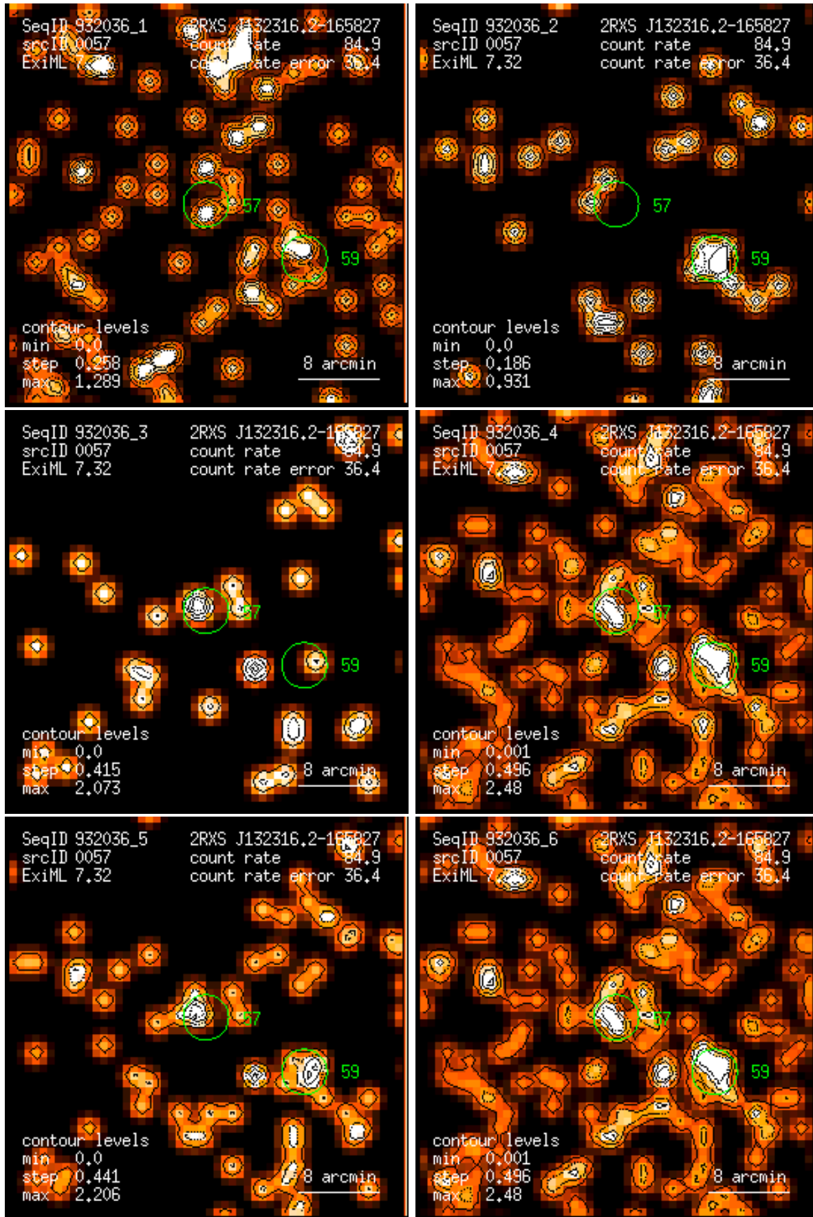
Figure 57: RASS 932036: detection 0057: band rate images, Gaussian filter: (1) PSPC channels 11 – 41, (2) 52 – 90, (3) 91 – 201, (4) 11 – 235, (5) 52 – 201, (6) 11 – 201. Broad band rates in counts/ks. Band rate contour levels in counts/ks/arcmin 2 .
