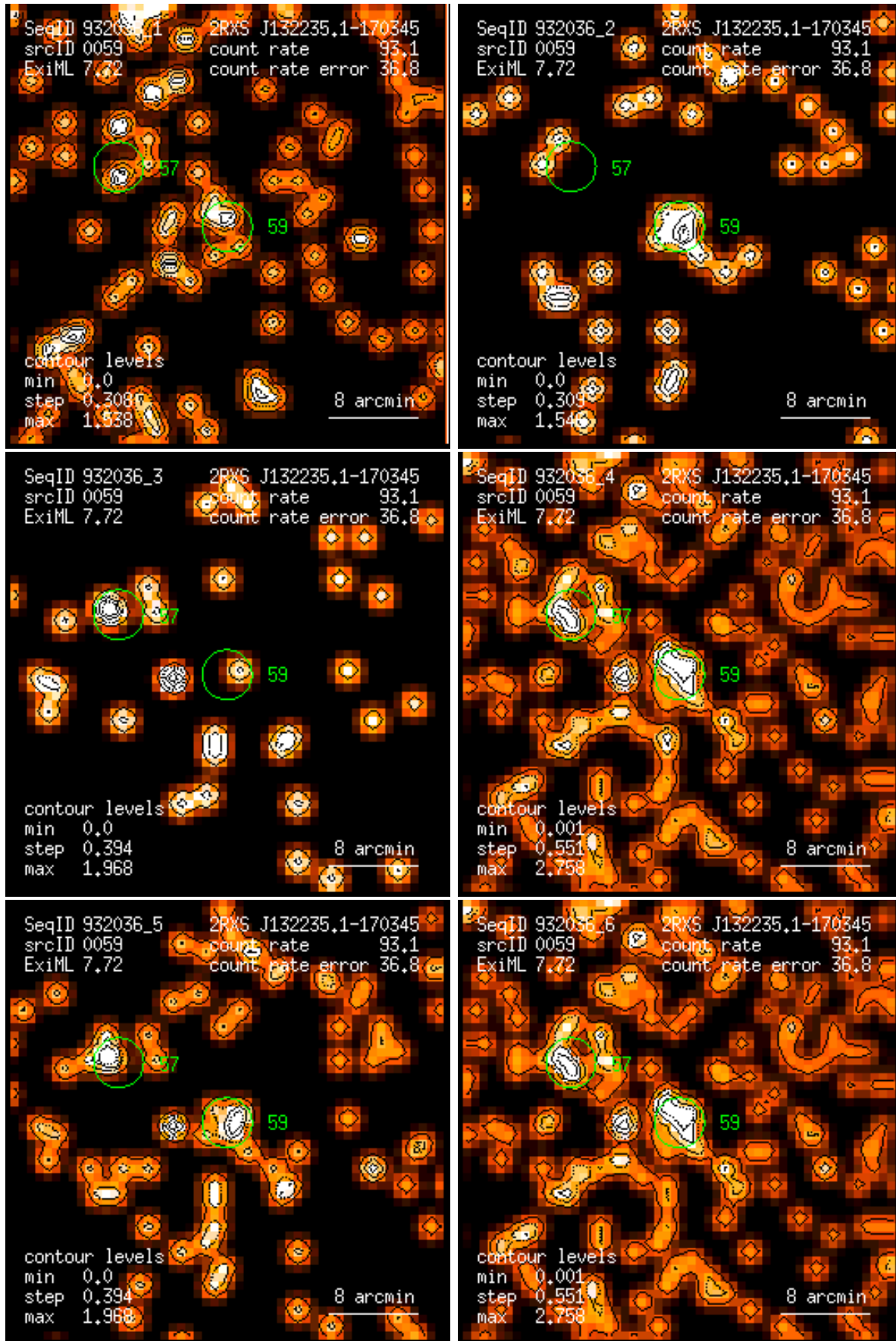
Figure 59: RASS 932036: detection 0059: band rate images, Gaussian filter: (1) PSPC channels 11 – 41, (2) 52 – 90, (3) 91 – 201, (4) 11 – 235, (5) 52 – 201, (6) 11 – 201. Broad band rates in counts/ks. Band rate contour levels in counts/ks/arcmin 2 .
