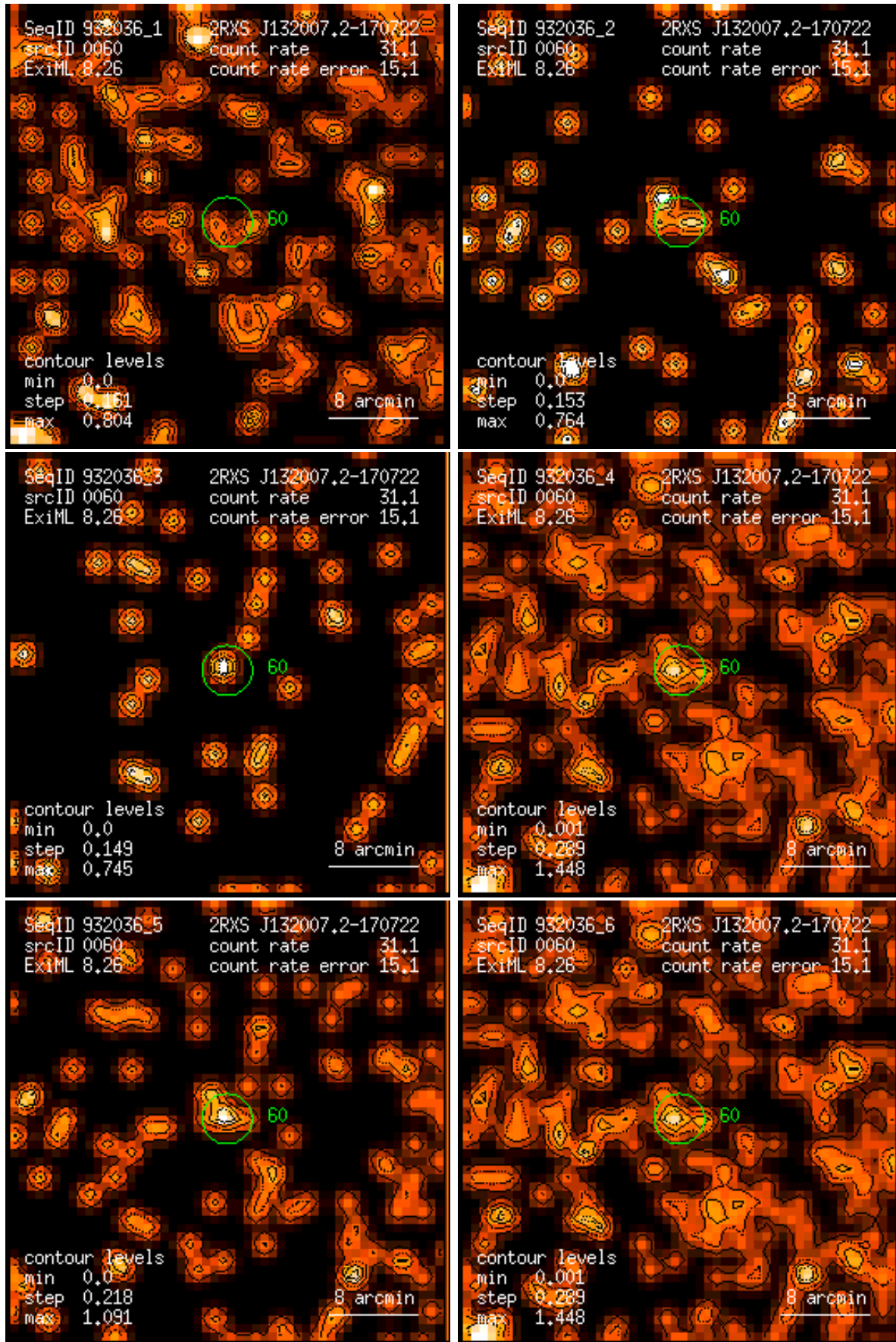
Figure 60: RASS 932036: detection 0060: band rate images, Gaussian filter: (1) PSPC channels 11 – 41, (2) 52 – 90, (3) 91 – 201, (4) 11 – 235, (5) 52 – 201, (6) 11 – 201. Broad band rates in counts/ks. Band rate contour levels in counts/ks/arcmin 2 .
