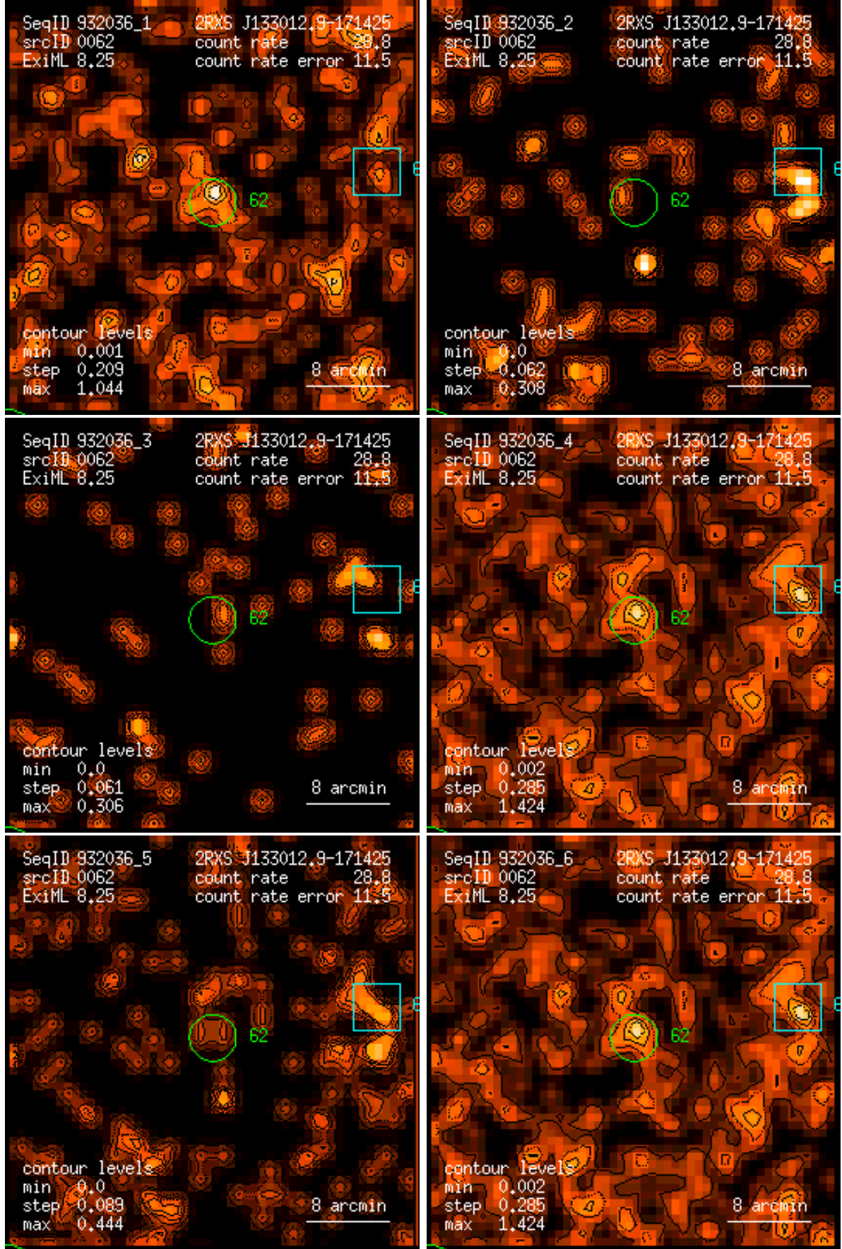
Figure 62: RASS 932036: detection 0062: band rate images, Gaussian filter: (1) PSPC channels 11 – 41, (2) 52 – 90, (3) 91 – 201, (4) 11 – 235, (5) 52 – 201, (6) 11 – 201. Broad band rates in counts/ks. Band rate contour levels in counts/ks/arcmin 2 .
