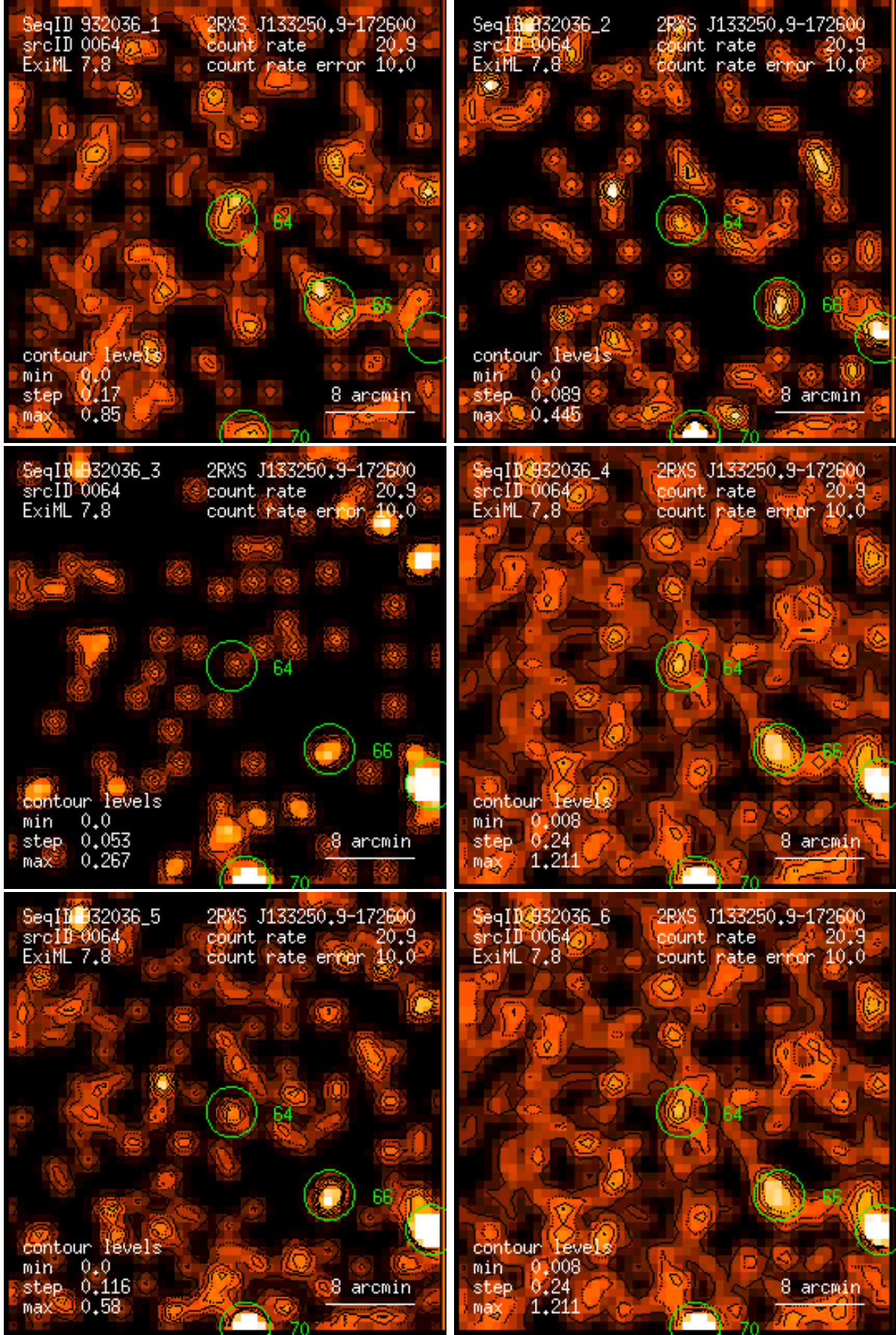
Figure 64: RASS 932036: detection 0064: band rate images, Gaussian filter: (1) PSPC channels 11 – 41, (2) 52 – 90, (3) 91 – 201, (4) 11 – 235, (5) 52 – 201, (6) 11 – 201. Broad band rates in counts/ks. Band rate contour levels in counts/ks/arcmin 2 .
