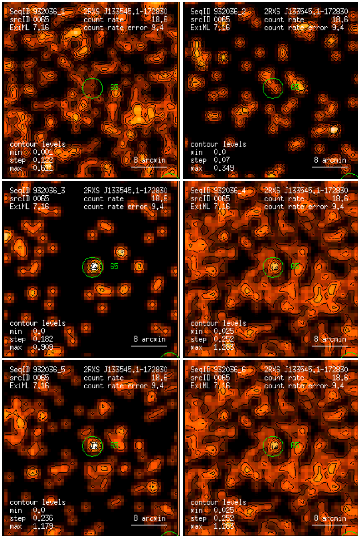
Figure 65: RASS 932036: detection 0065: band rate images, Gaussian filter: (1) PSPC channels 11 – 41, (2) 52 – 90, (3) 91 – 201, (4) 11 – 235, (5) 52 – 201, (6) 11 – 201. Broad band rates in counts/ks. Band rate contour levels in counts/ks/arcmin 2 .
