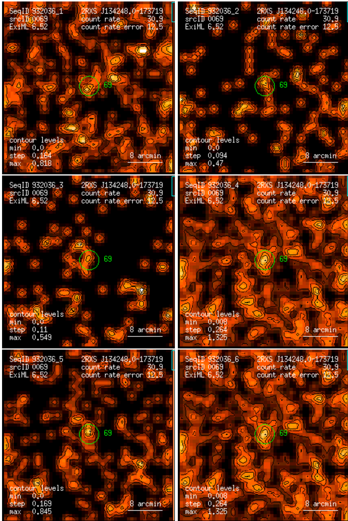
Figure 69: RASS 932036: detection 0069: band rate images, Gaussian filter: (1) PSPC channels 11 – 41, (2) 52 – 90, (3) 91 – 201, (4) 11 – 235, (5) 52 – 201, (6) 11 – 201. Broad band rates in counts/ks. Band rate contour levels in counts/ks/arcmin 2 .
