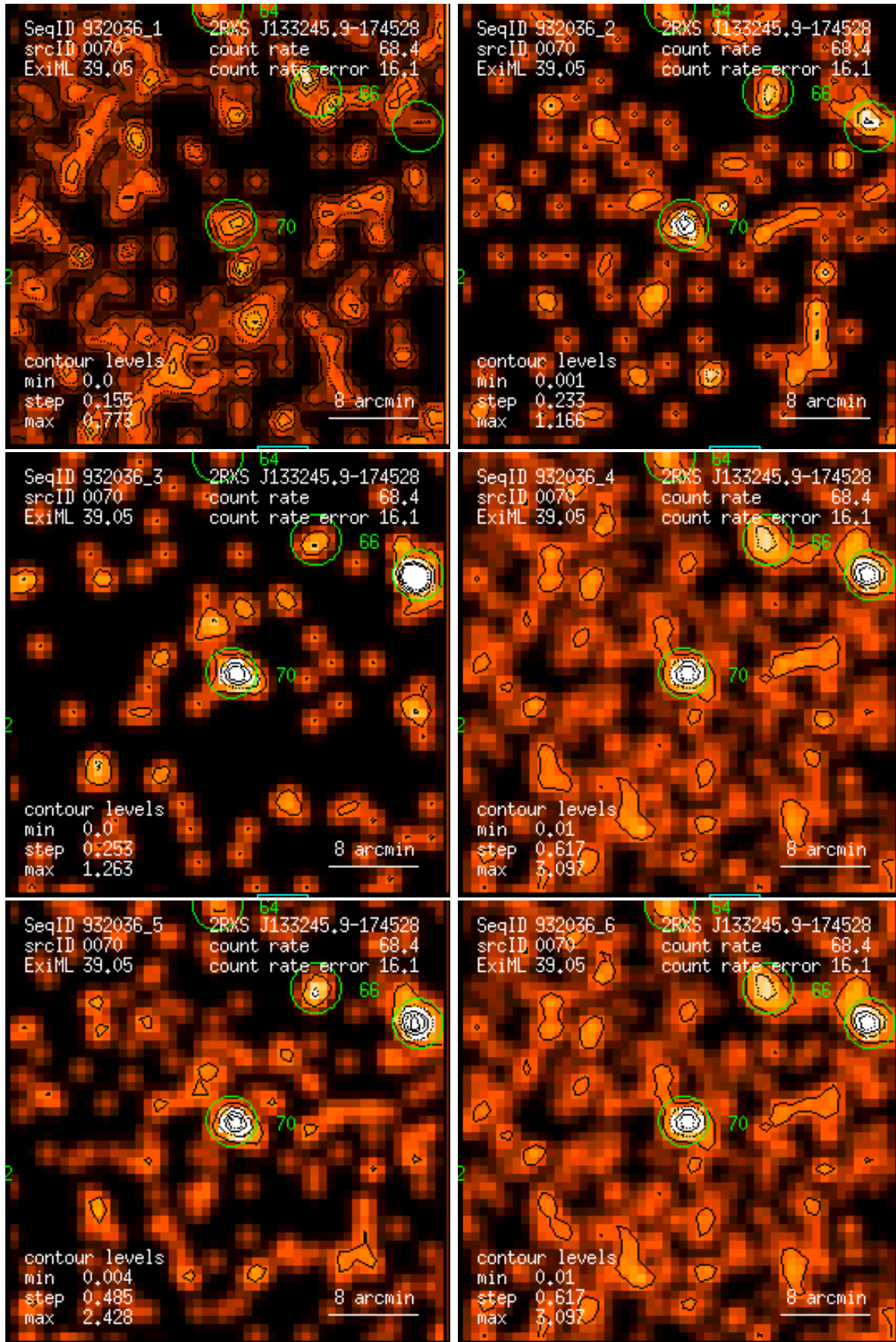
Figure 70: RASS 932036: detection 0070: band rate images, Gaussian filter: (1) PSPC channels 11 – 41, (2) 52 – 90, (3) 91 – 201, (4) 11 – 235, (5) 52 – 201, (6) 11 – 201. Broad band rates in counts/ks. Band rate contour levels in counts/ks/arcmin 2 .
