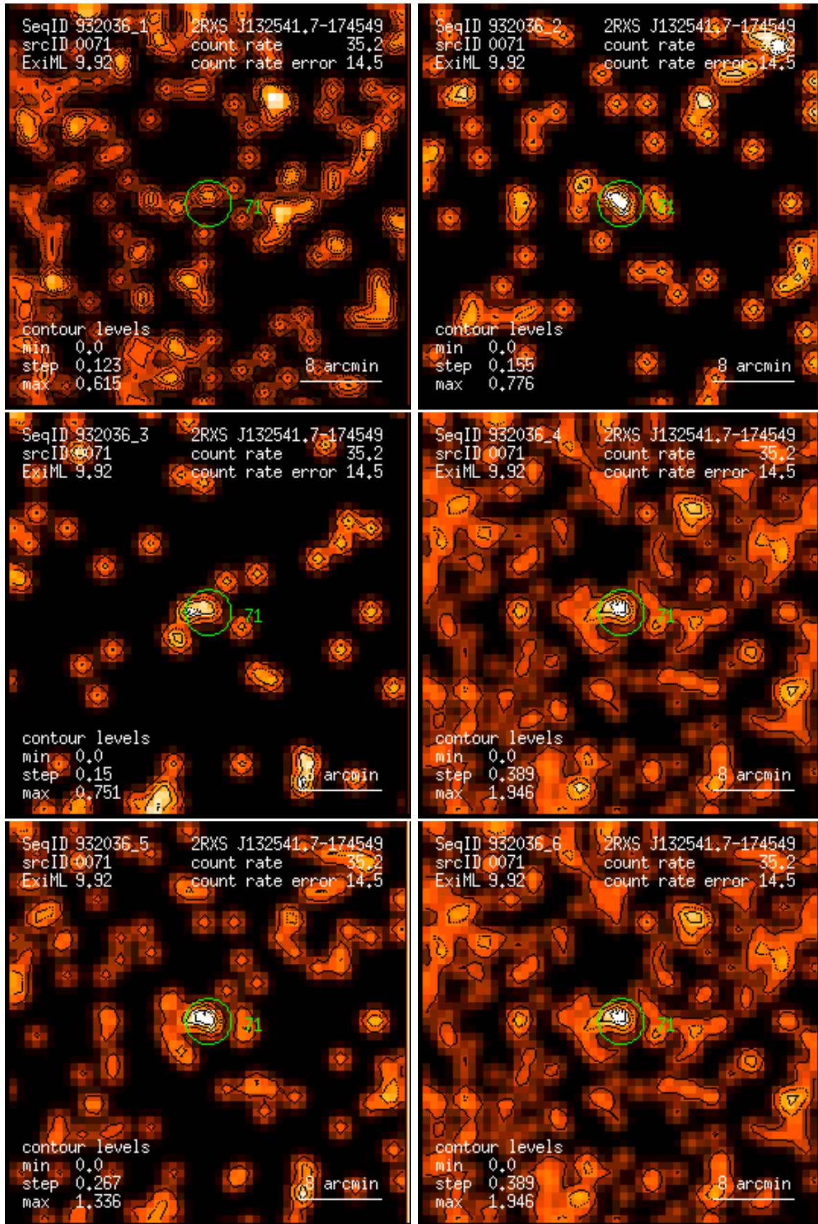
Figure 71: RASS 932036: detection 0071: band rate images, Gaussian filter: (1) PSPC channels 11 – 41, (2) 52 – 90, (3) 91 – 201, (4) 11 – 235, (5) 52 – 201, (6) 11 – 201. Broad band rates in counts/ks. Band rate contour levels in counts/ks/arcmin 2 .
