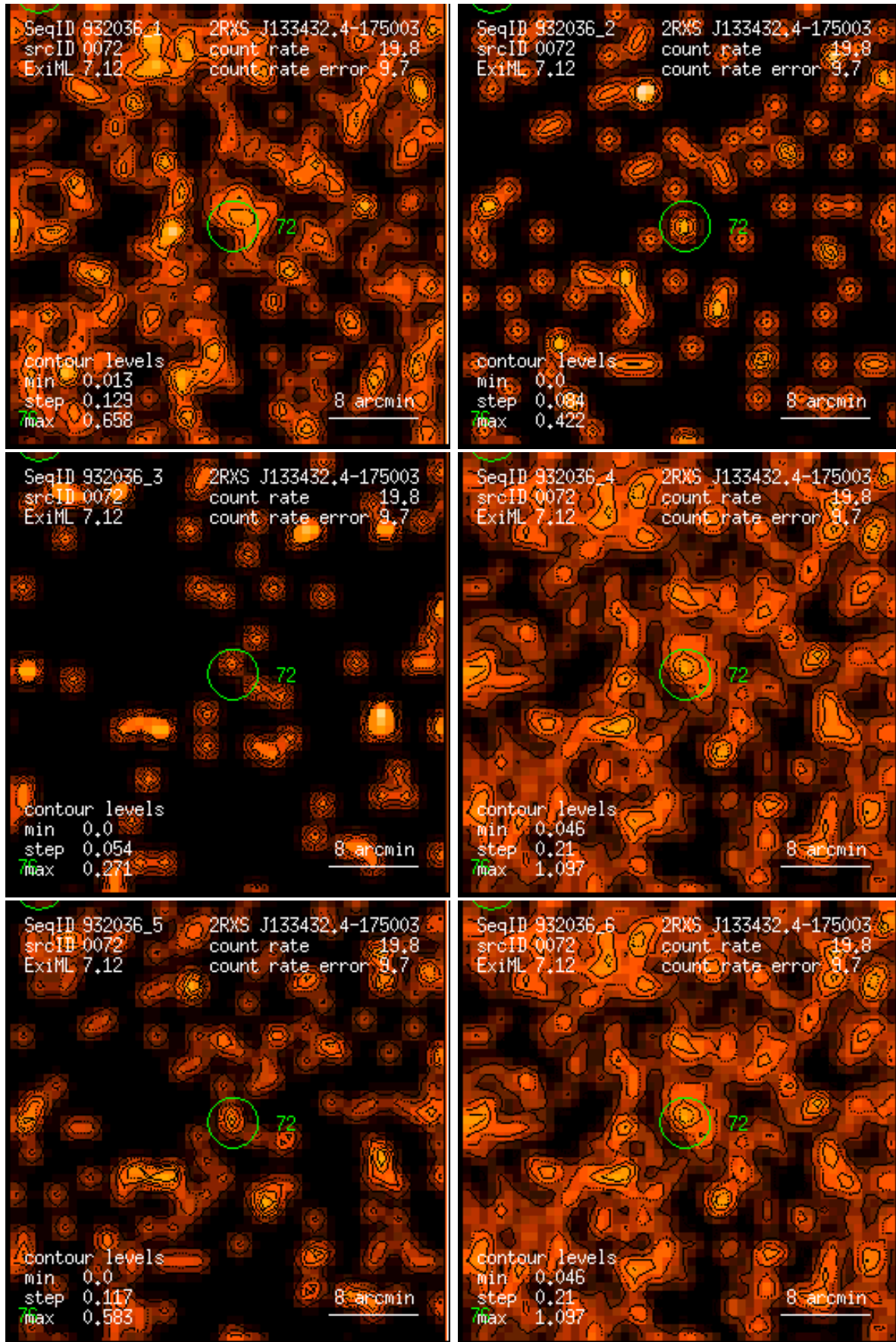
Figure 72: RASS 932036: detection 0072: band rate images, Gaussian filter: (1) PSPC channels 11 – 41, (2) 52 – 90, (3) 91 – 201, (4) 11 – 235, (5) 52 – 201, (6) 11 – 201. Broad band rates in counts/ks. Band rate contour levels in counts/ks/arcmin 2 .
