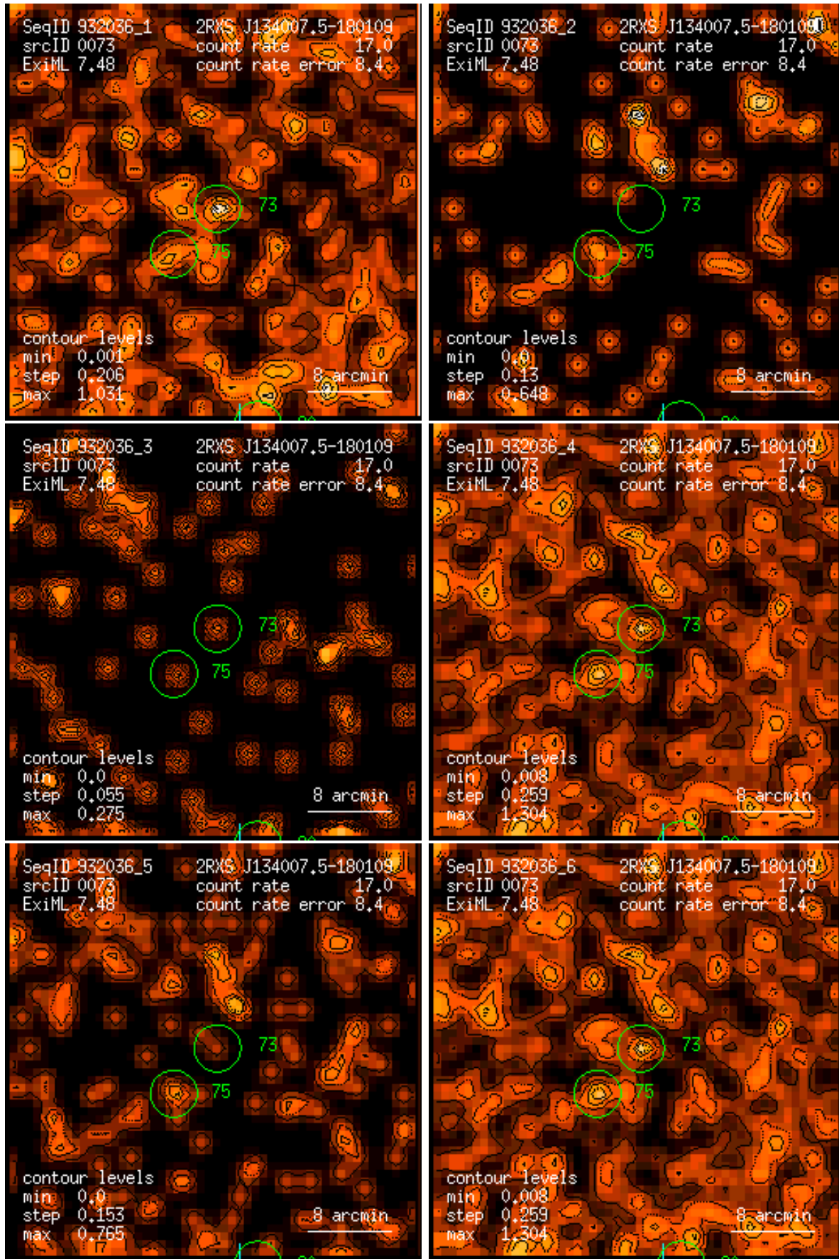
Figure 73: RASS 932036: detection 0073: band rate images, Gaussian filter: (1) PSPC channels 11 – 41, (2) 52 – 90, (3) 91 – 201, (4) 11 – 235, (5) 52 – 201, (6) 11 – 201. Broad band rates in counts/ks. Band rate contour levels in counts/ks/arcmin 2 .
