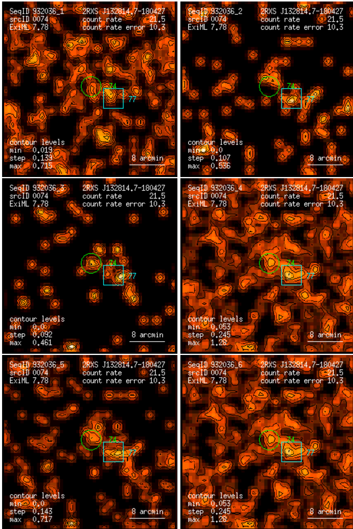
Figure 74: RASS 932036: detection 0074: band rate images, Gaussian filter: (1) PSPC channels 11 – 41, (2) 52 – 90, (3) 91 – 201, (4) 11 – 235, (5) 52 – 201, (6) 11 – 201. Broad band rates in counts/ks. Band rate contour levels in counts/ks/arcmin 2 .
