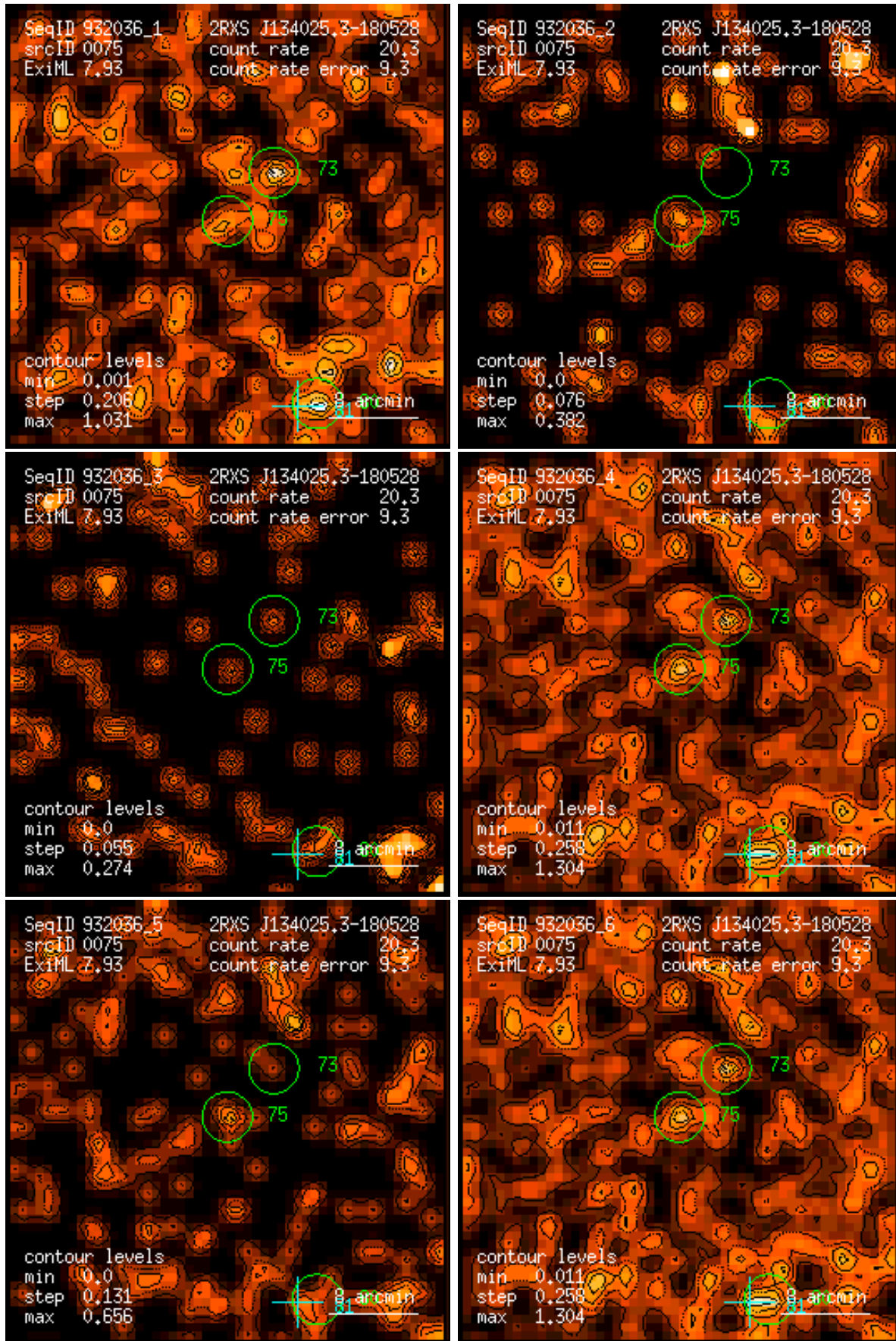
Figure 75: RASS 932036: detection 0075: band rate images, Gaussian filter: (1) PSPC channels 11 – 41, (2) 52 – 90, (3) 91 – 201, (4) 11 – 235, (5) 52 – 201, (6) 11 – 201. Broad band rates in counts/ks. Band rate contour levels in counts/ks/arcmin 2 .
