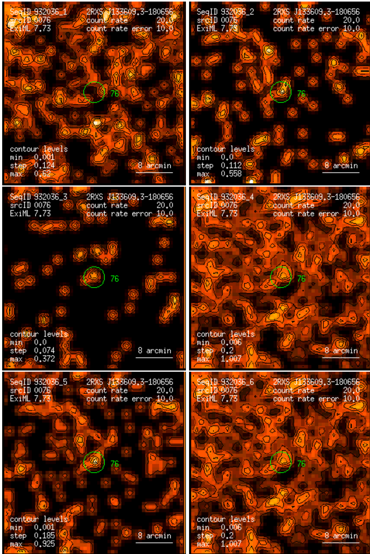
Figure 76: RASS 932036: detection 0076: band rate images, Gaussian filter: (1) PSPC channels 11 – 41, (2) 52 – 90, (3) 91 – 201, (4) 11 – 235, (5) 52 – 201, (6) 11 – 201. Broad band rates in counts/ks. Band rate contour levels in counts/ks/arcmin 2 .
