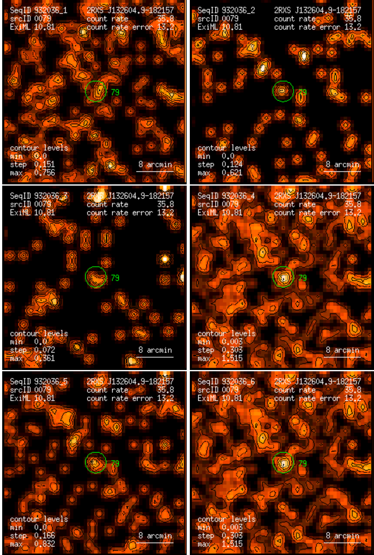
Figure 79: RASS 932036: detection 0079: band rate images, Gaussian filter: (1) PSPC channels 11 – 41, (2) 52 – 90, (3) 91 – 201, (4) 11 – 235, (5) 52 – 201, (6) 11 – 201. Broad band rates in counts/ks. Band rate contour levels in counts/ks/arcmin 2 .
