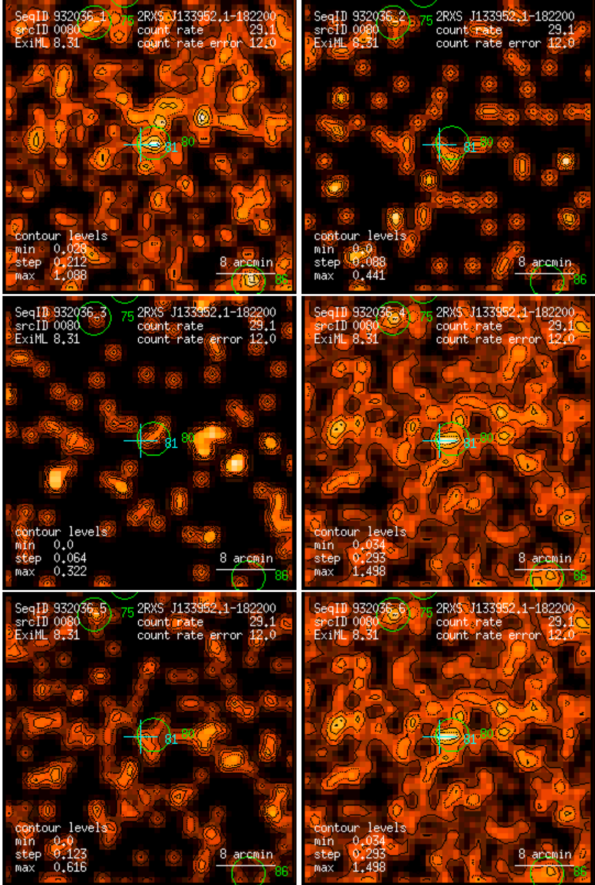
Figure 80: RASS 932036: detection 0080: band rate images, Gaussian filter: (1) PSPC channels 11 – 41, (2) 52 – 90, (3) 91 – 201, (4) 11 – 235, (5) 52 – 201, (6) 11 – 201. Broad band rates in counts/ks. Band rate contour levels in counts/ks/arcmin 2 .
