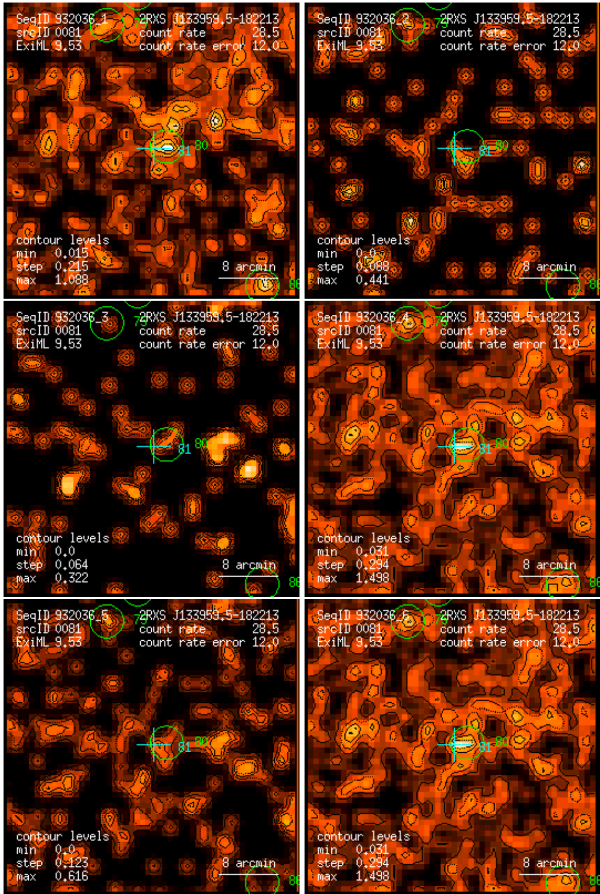
Figure 81: RASS 932036: detection 0081: band rate images, Gaussian filter: (1) PSPC channels 11 – 41, (2) 52 – 90, (3) 91 – 201, (4) 11 – 235, (5) 52 – 201, (6) 11 – 201. Broad band rates in counts/ks. Band rate contour levels in counts/ks/arcmin 2 .
