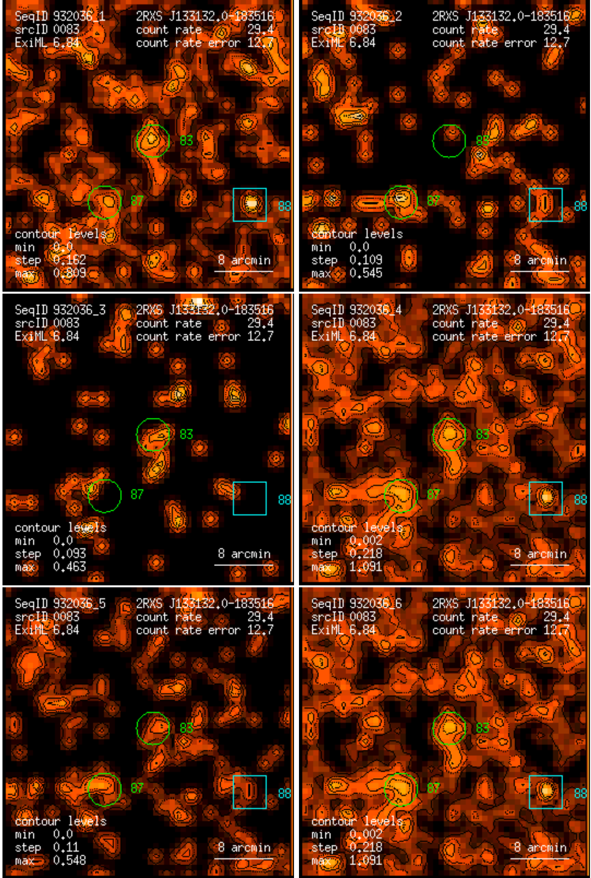
Figure 83: RASS 932036: detection 0083: band rate images, Gaussian filter: (1) PSPC channels 11 – 41, (2) 52 – 90, (3) 91 – 201, (4) 11 – 235, (5) 52 – 201, (6) 11 – 201. Broad band rates in counts/ks. Band rate contour levels in counts/ks/arcmin 2 .
