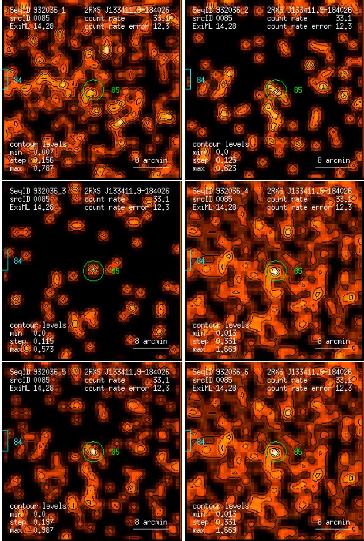
Figure 85: RASS 932036: detection 0085: band rate images, Gaussian filter: (1) PSPC channels 11 – 41, (2) 52 – 90, (3) 91 – 201, (4) 11 – 235, (5) 52 – 201, (6) 11 – 201. Broad band rates in counts/ks. Band rate contour levels in counts/ks/arcmin 2 .
