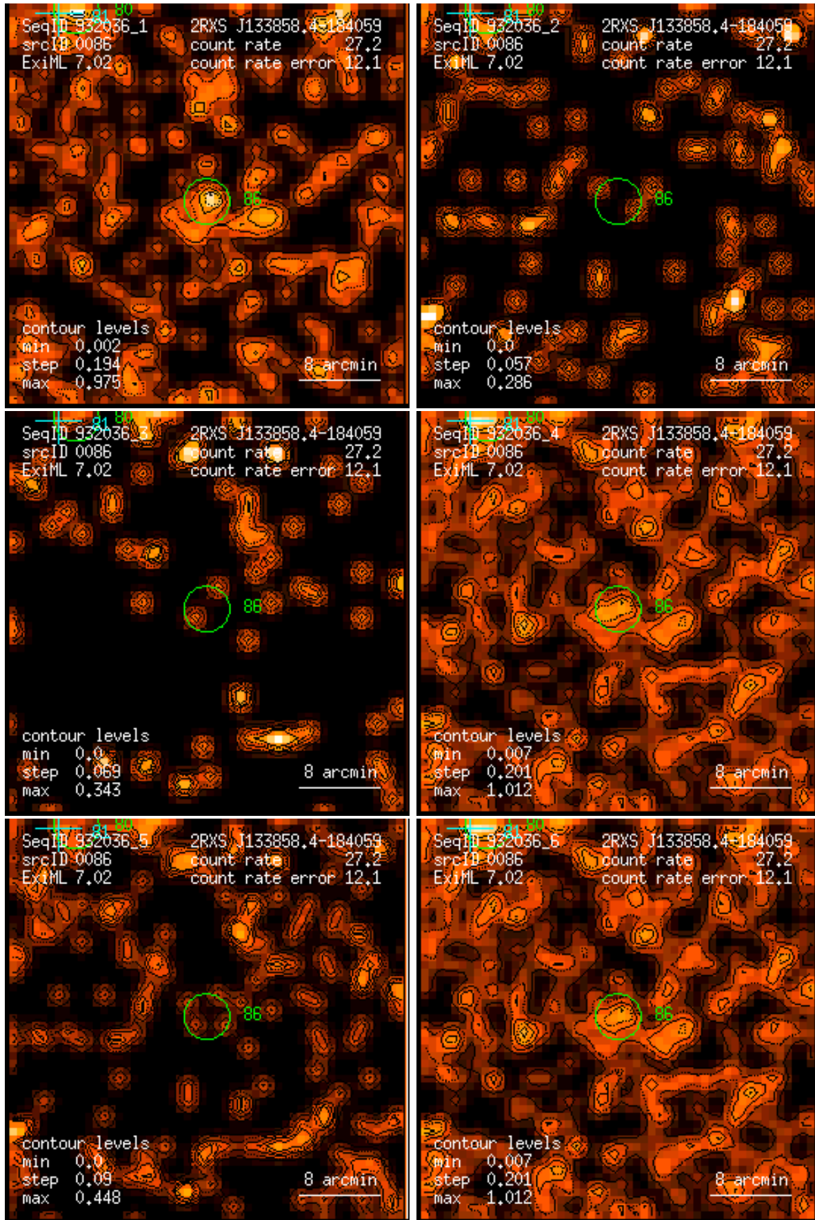
Figure 86: RASS 932036: detection 0086: band rate images, Gaussian filter: (1) PSPC channels 11 – 41, (2) 52 – 90, (3) 91 – 201, (4) 11 – 235, (5) 52 – 201, (6) 11 – 201. Broad band rates in counts/ks. Band rate contour levels in counts/ks/arcmin 2 .
